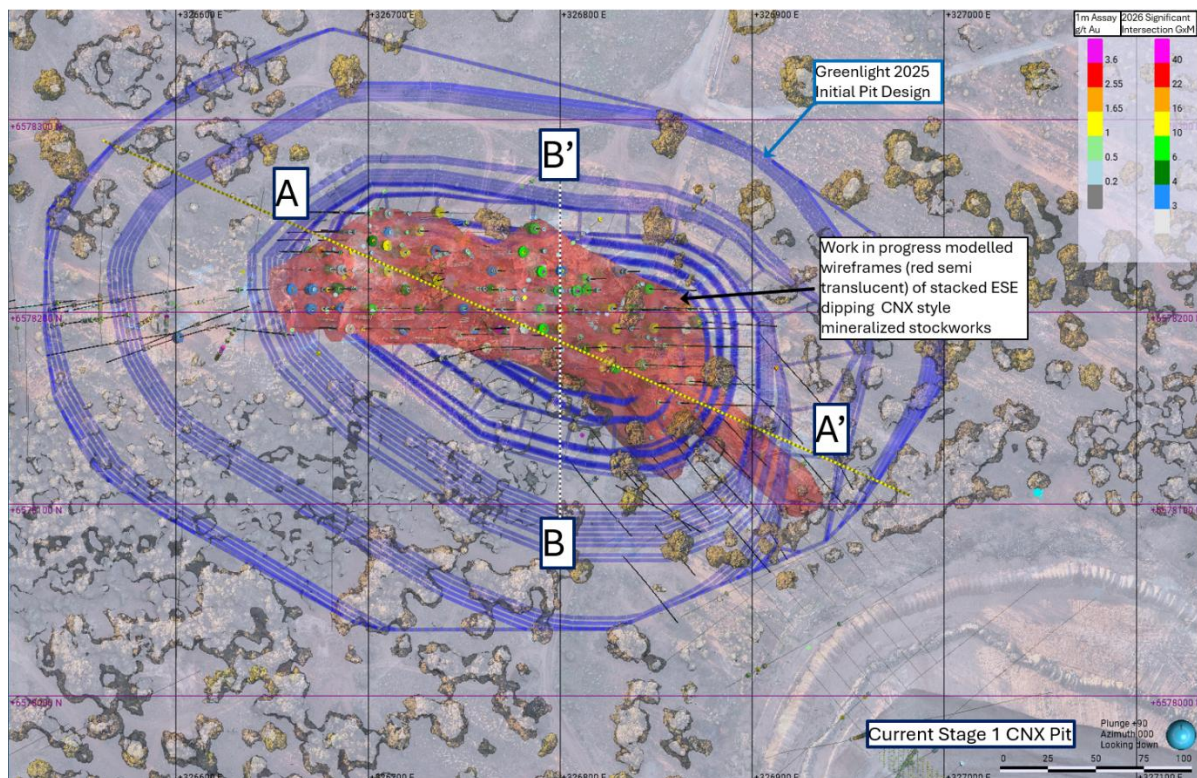
Figure 2: Plan view Green Light deposit modelled mineralisation (Red wireframes) dip moderately to the East within the E-W striking G2 Gabbro. Long section line location A-A' for Figure 3 is shown with yellow dashed line. Cross section line location B-B' for Figure 4 is shown with white dashed line. Initial 2025 Green Light Pit design stings are coloured dark blue. 2026 drilling comprises 20m x 20m infill RC drilling targeting the volume most likely to be amenable to open pit extraction.
