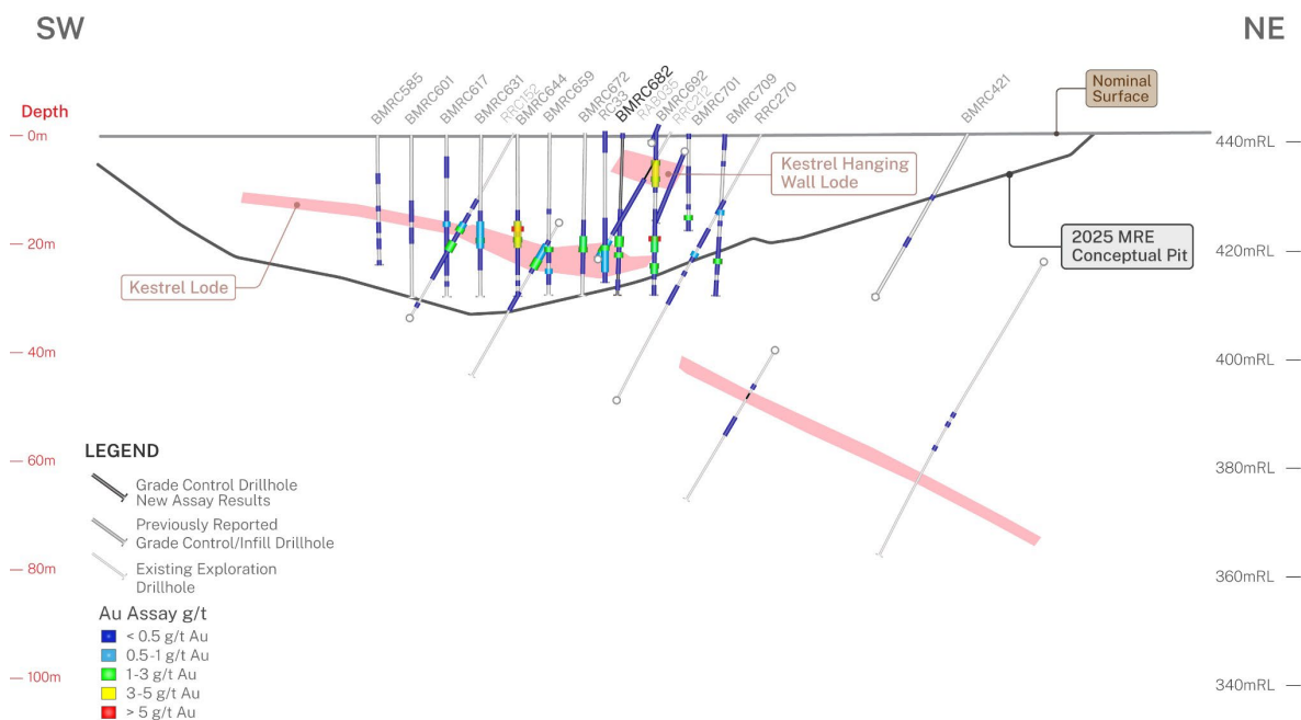
Figure 8. Queen Alexandra Section 7-7'
