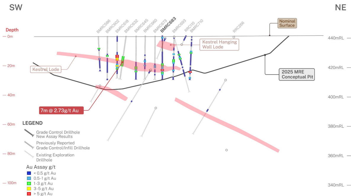
Figure 9. Queen Alexandra Section 8-8'
