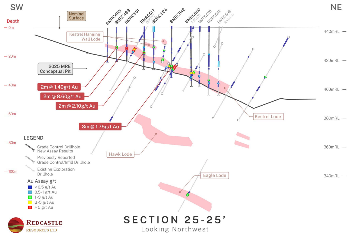
Figure 25. Queen Alexandra Section 25-25'
