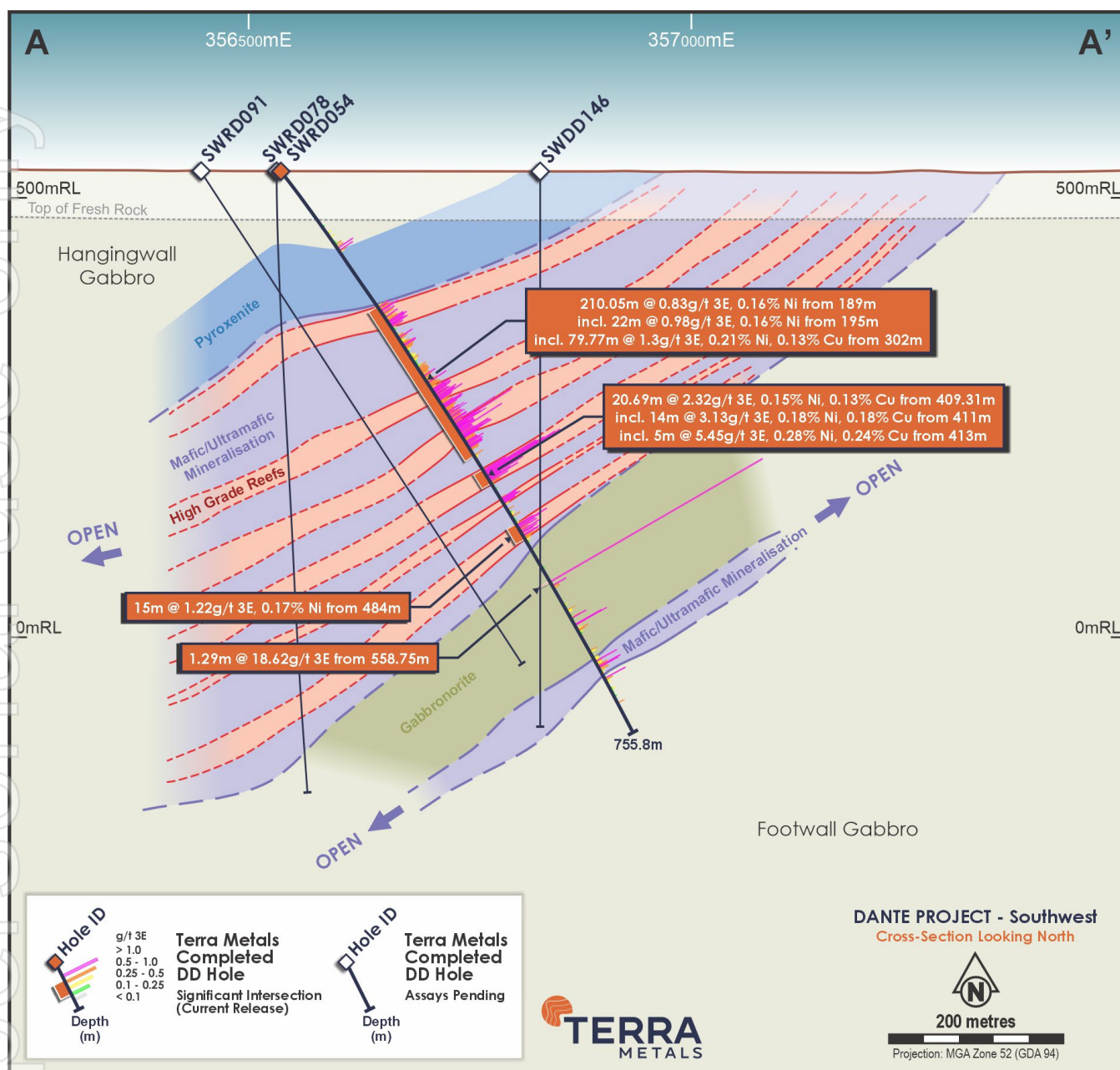
Figure 2. Cross-section A-A' through the Southwest Main Sulfide Zone including the currently reported diamond tail and previously reported RC pre-collar for SWRD054 with interpreted mineralised envelopes. The envelopes are conceptual and based on current drilling, geological logging and structural data.
