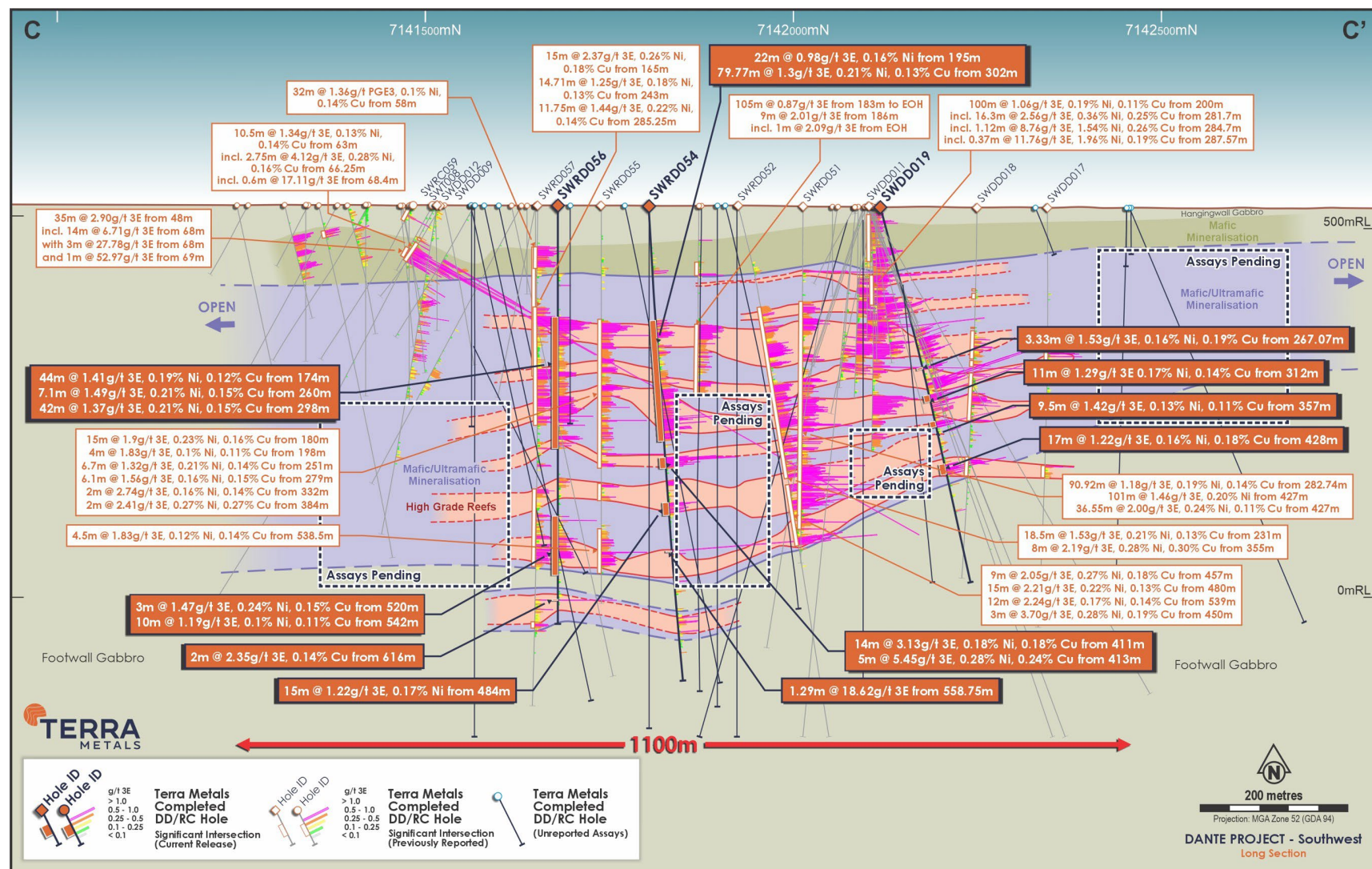
Figure 4. Long-section C-C' through the Southwest Main Sulfide Zone showing the interpreted geology and high-grade reefs hosted within the Jameson Layered Mafic Complex. The interpretations are conceptual and based on current drilling, geological logging and structural data.
