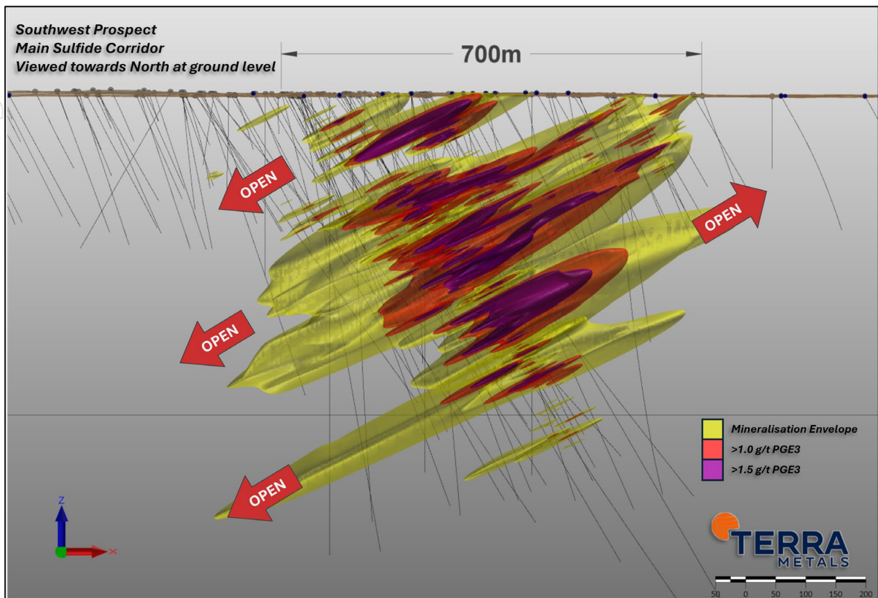
Figure 5. 3D view of Southwest Project viewed from the south, showing the interpreted mineralisation envelope and high-grade reefs interpreted from current drill results.
