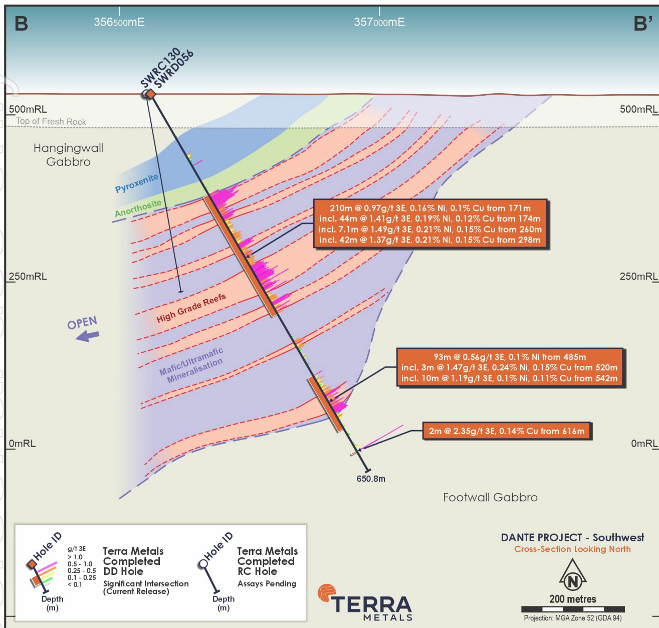
Figure 3. Cross-section B-B' through the Southwest Main Sulfide Zone including the currently reported diamond tail and previously reported RC pre-collar for SWRD056 with interpreted mineralised envelopes. The envelopes are conceptual and based on current drilling, geological logging and structural data.
