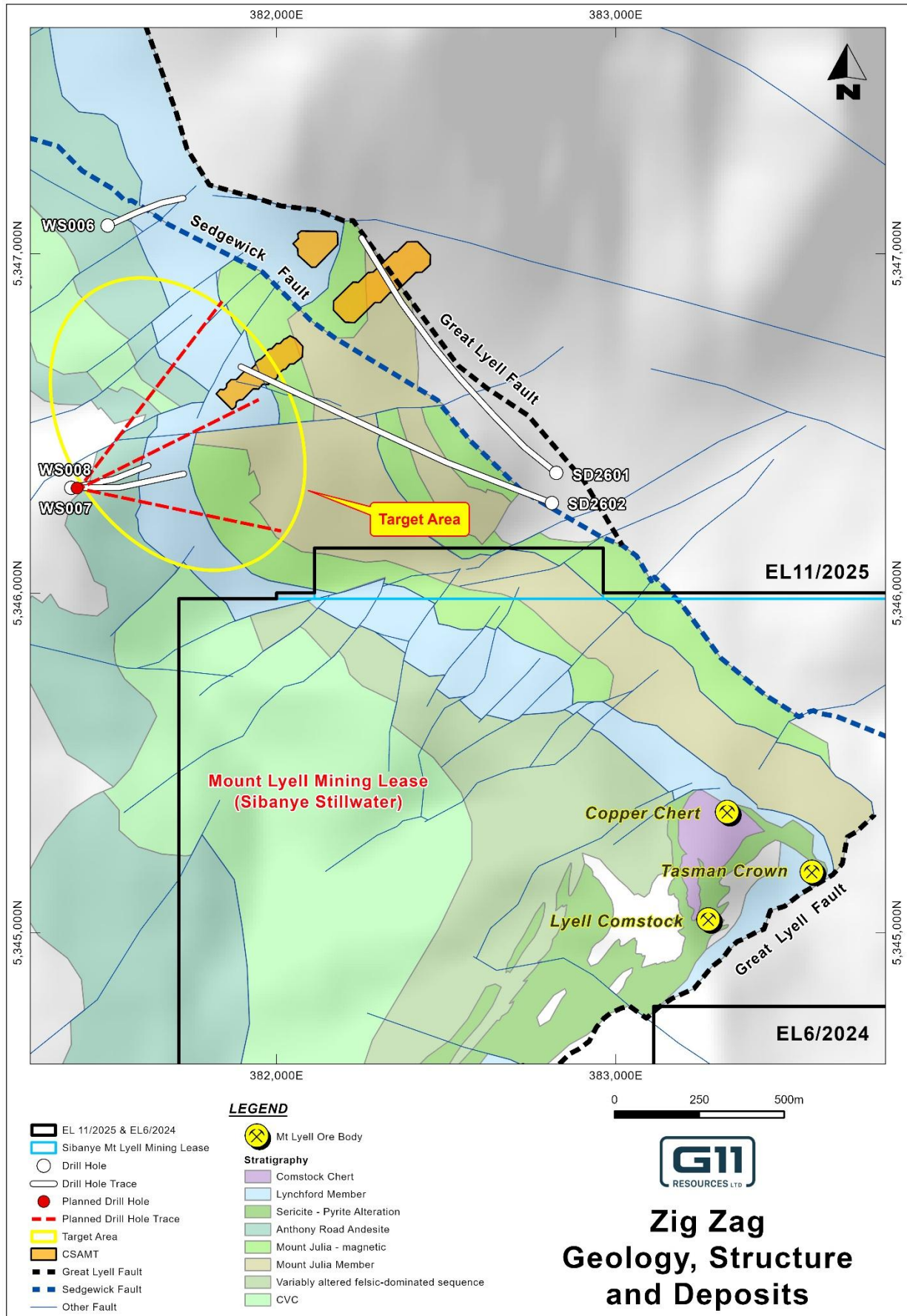
Figure 2 – Updated geological interpretation with proposed drillhole locations at Zig Zag Hill.
