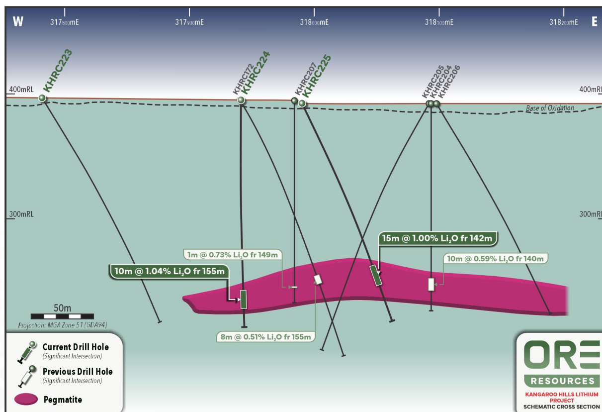
Figure 2: Cross Section – KHRC224 to KHRC225
