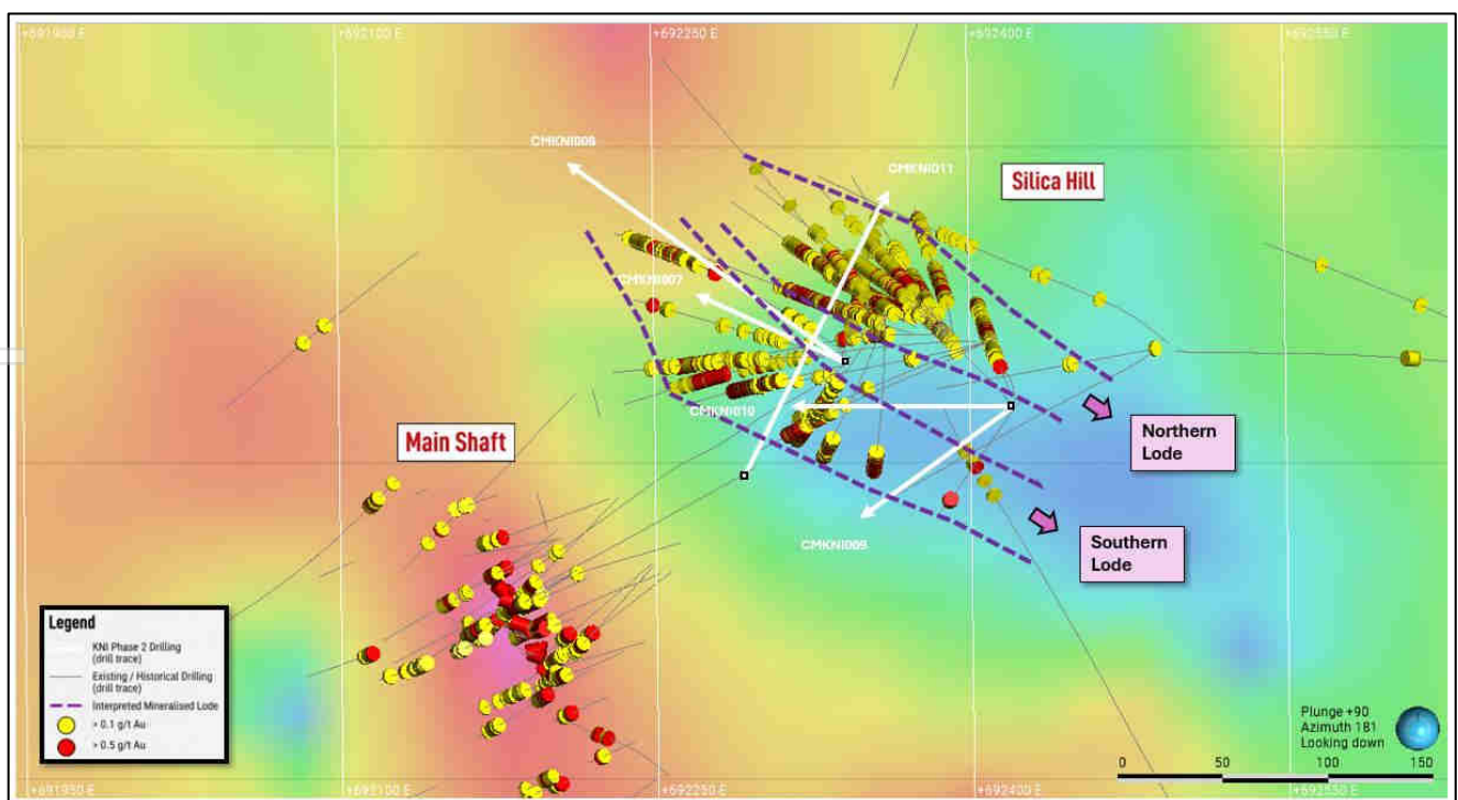
Figure 3: Plan view of the Silica Hill prospect showing Phase 2 diamond drilling (white traces) and historical drilling over processed gravity imagery. The interpreted Northern and Southern Lodges are shown in purple, highlighting the relationship between known mineralisation and the margin of the prominent gravity low. Phase 2 drilling is systematically testing the lateral and depth extent of the Silica Hill mineralised system.
