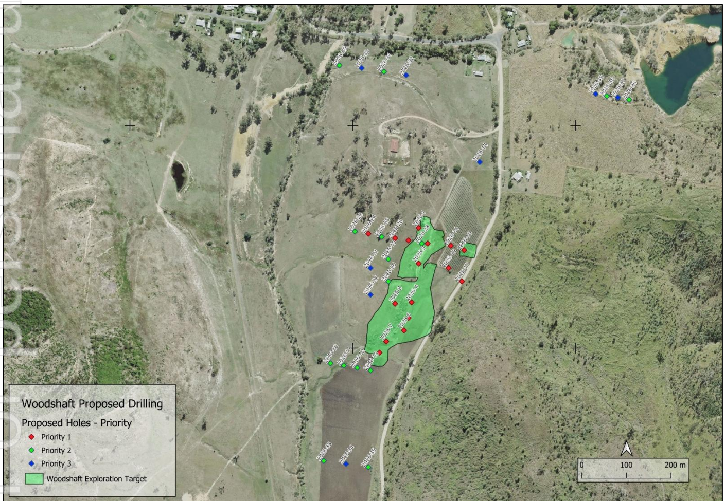
Figure 4: Plan view showing the Woods Shaft Resource and planned holes in proximity to the Mt Chalmers historic open pit.
