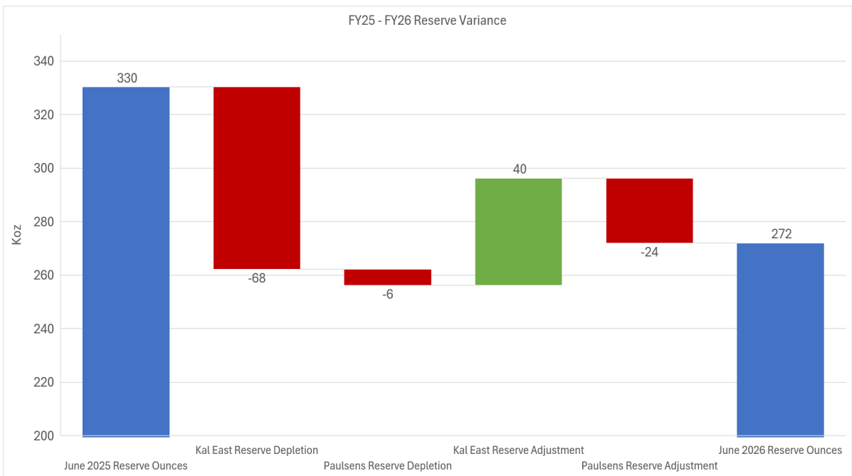
Figure 2: Reserve variance FY25 / FY26 waterfall chart
