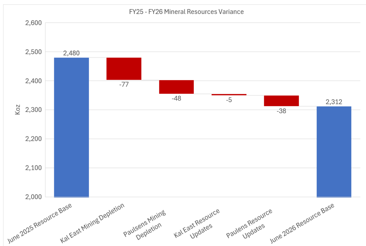
Figure 1: Resource variance FY25 / FY26 waterfall chart
