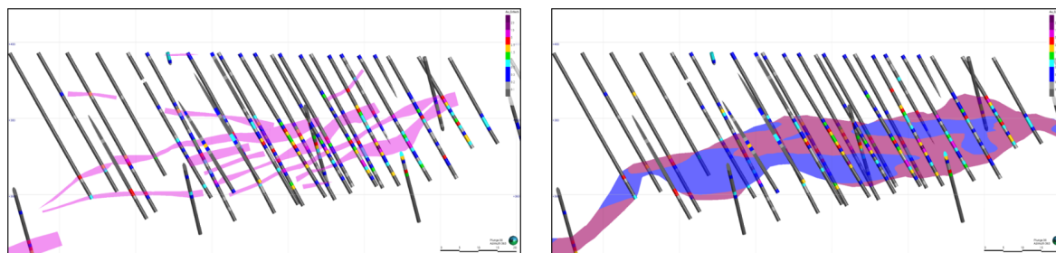
Figure 3: Updated Fingals mineralisation interpretation (2021 MRE - Left; 2026 MRE - Right)
