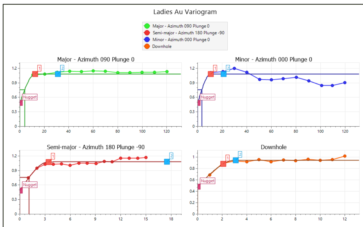
Figure 9: Variogram Models
