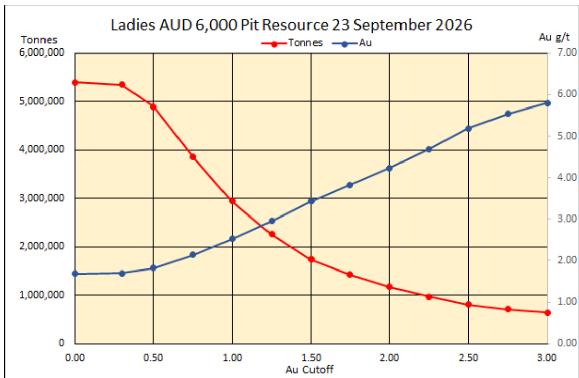
Figure 13: Optimal Grade Tonnage Curve for the Ladies (Measured + Indicated + Inferred)
