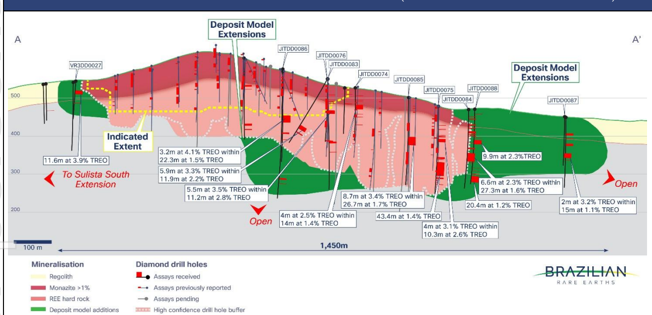
FIGURE 5: SULISTA EAST INFILL AND STEP-OUT DRILLING (LONGSECTION VIEW TO THE NW)
