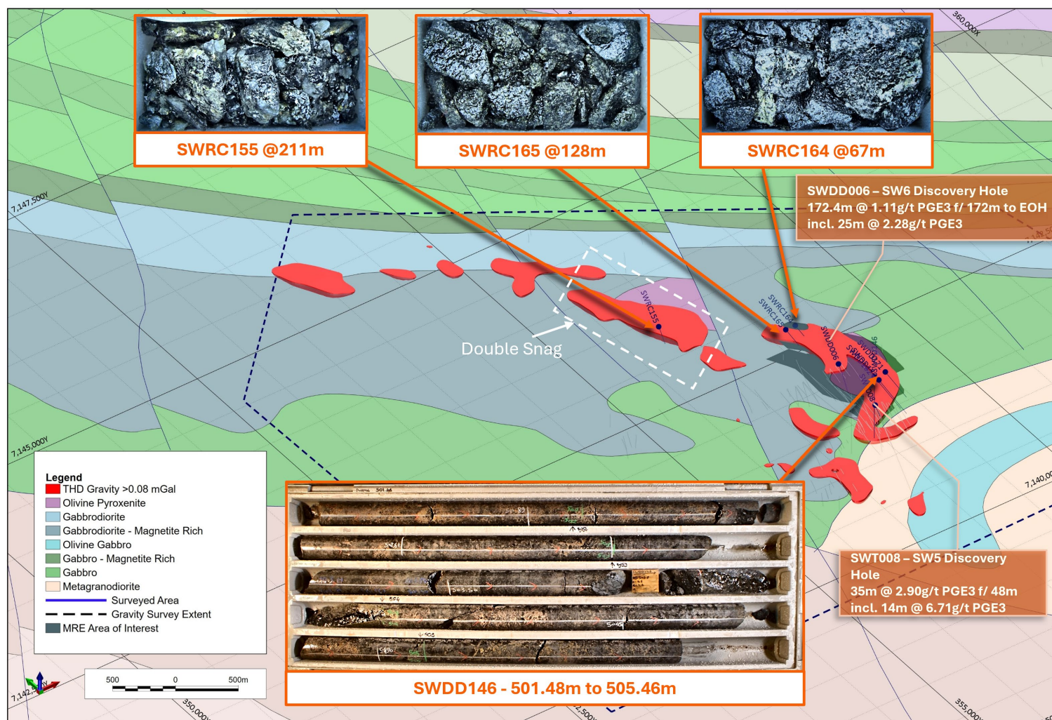
Figure 4. New interpretation of the Southwest Igneous Complex, showing newly interpreted geology and structural map, along with newly defined THD-Gravity geophysical data. Also shown are the locations of drillholes that successfully intersected sulfide mineralisation. Visual estimates only; not a substitute for laboratory assays. Assays pending.
