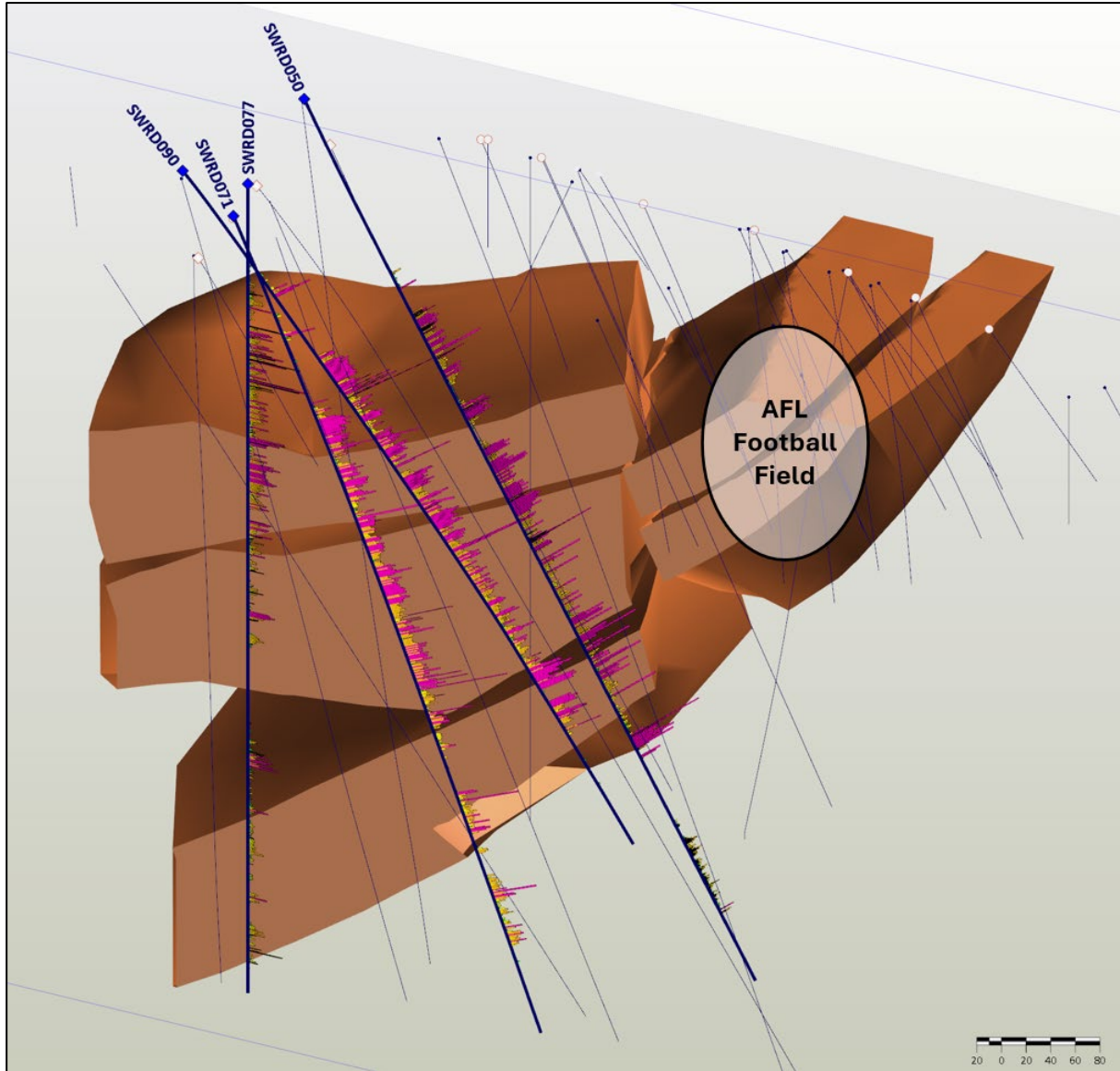
Figure 2. Oblique 3D cross-section of the Southwest mineralisation model showing the drillholes reported in this announcement, with PGE grade shown in bar graph form, together with an indicative AFL football field for scale (approximately 165 m x 135 m).
