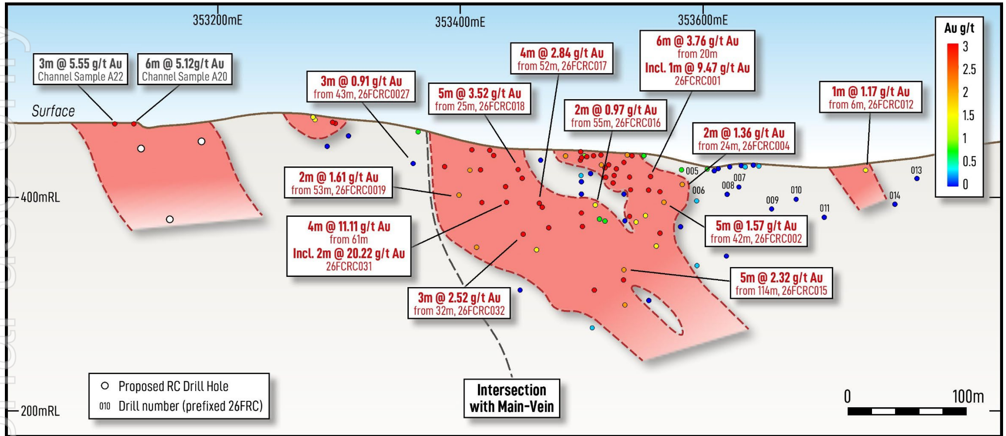
Figure 4. Long section across the Francis Creek A Vein drilling, showing the results from the A Vein east of the Main Vein and limited testing of the A Vein West area.
