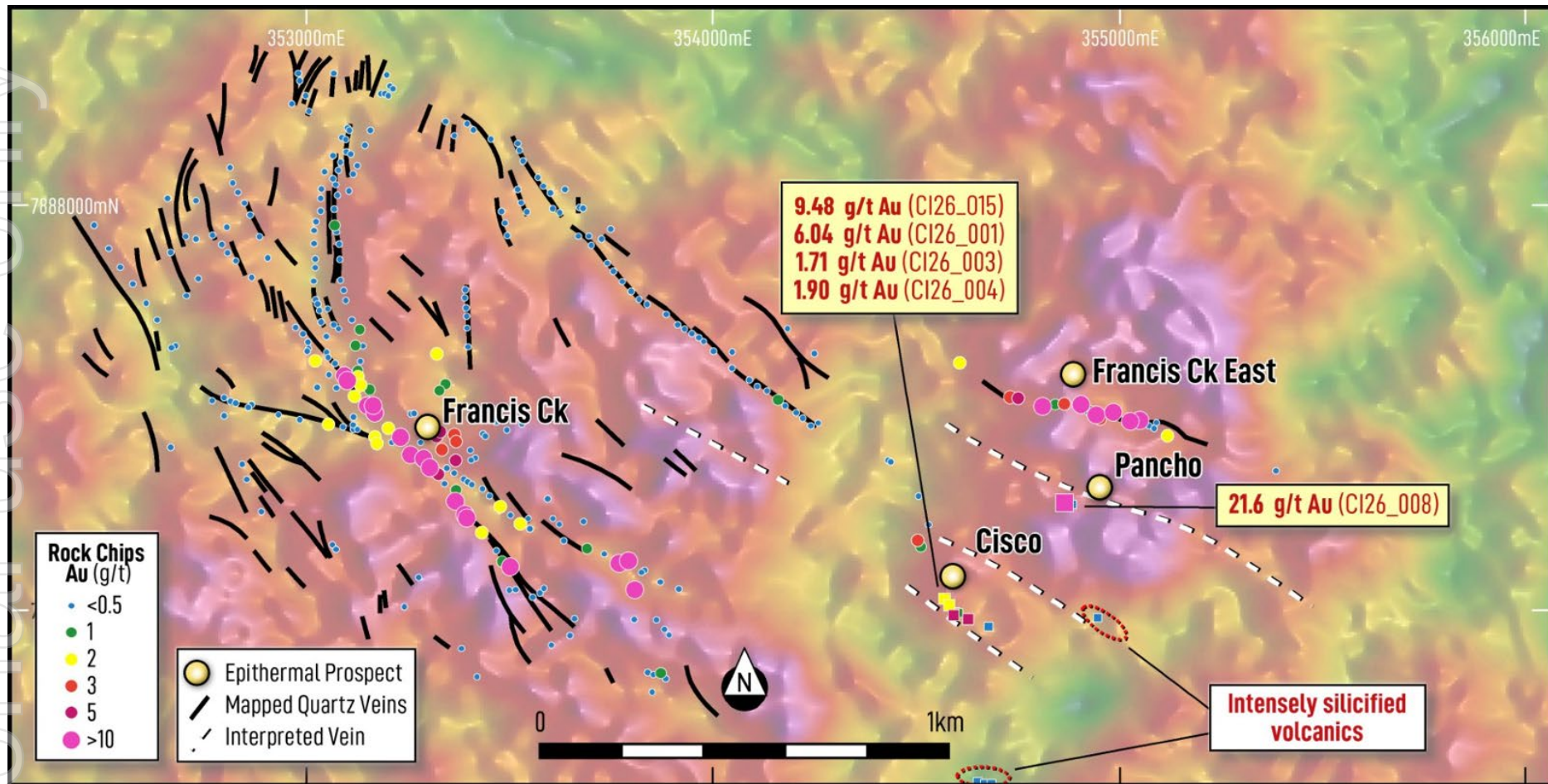
Figure 7: Radiometric image with zones of potassium depletion correlating to mapped quartz veins (black) in the Francis Creek to Francis Creek East area. Interpreted and now ground truthed, veins (white) including Cisco and Pancho veins show elevated Au in rock chip sampling.
