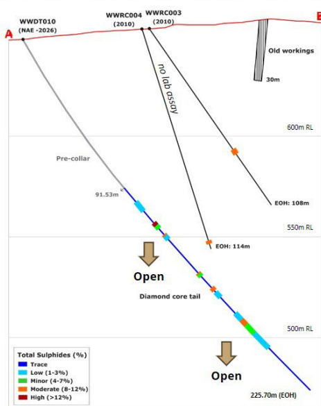
Figure 2 – Location and cross-section through WWRC010/WWDT010 showing logged total sulphides and vein sets
