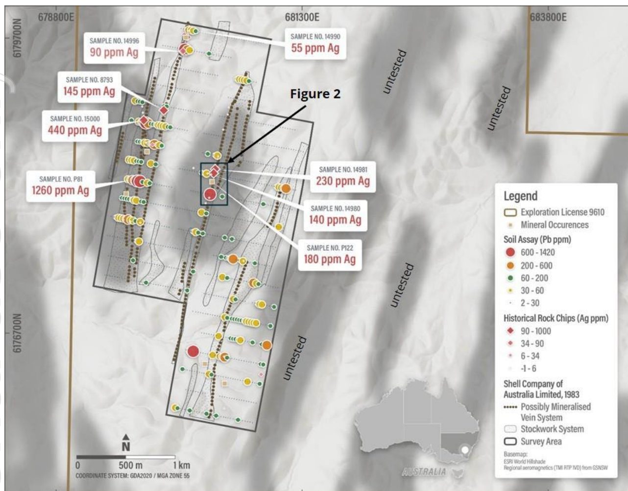
Figure 1 - Historic soil survey results (lead, ppm) and rock chip results (silver, ppm) and mapped geology - overlain on aeromagnetic data (1 st vertical derivative), Wallah Silver Project, NSW (refer also to the ASX announcement dated 2 March 2026). See box for location of Figure 2.
