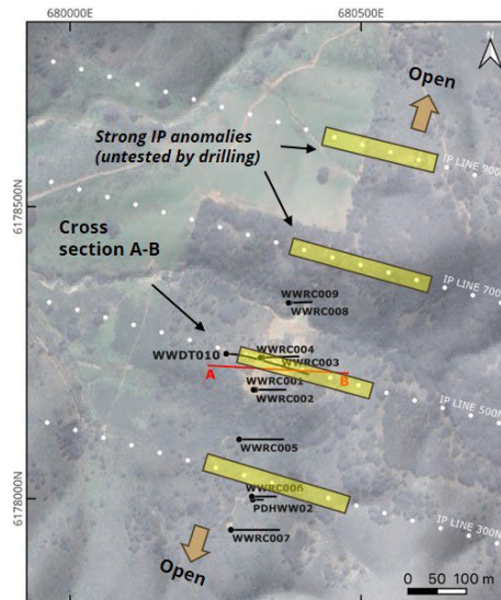
Figure 2 – Location and cross-section through WWRC010/WWDT010 showing logged total sulphides and vein sets
