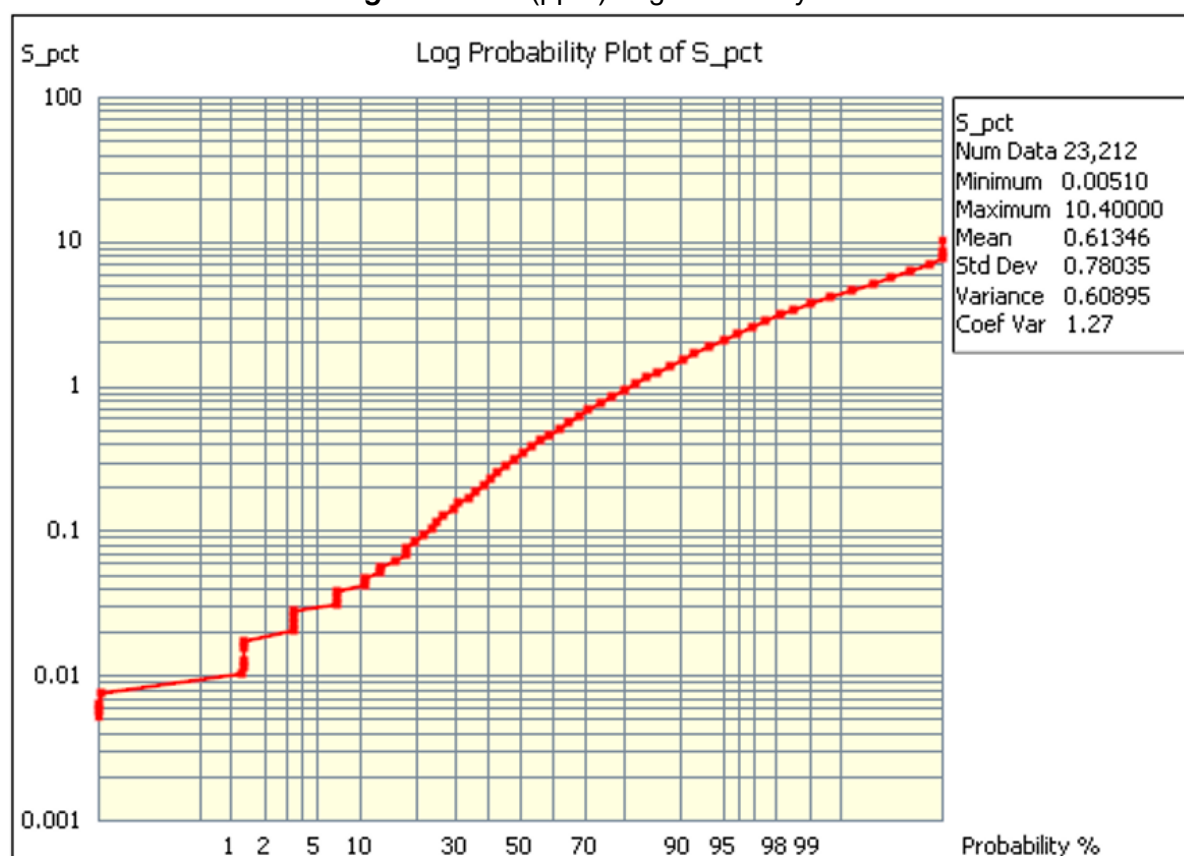
Figure 13: S (%) Log Probability Plot
