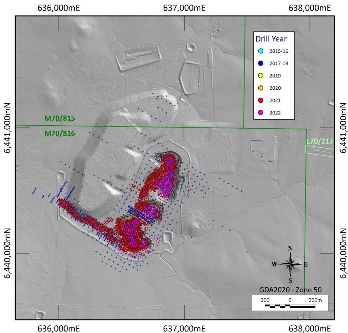
Figure 5: Tampia Project Drill Holes by Year used in the 2026 MRE
