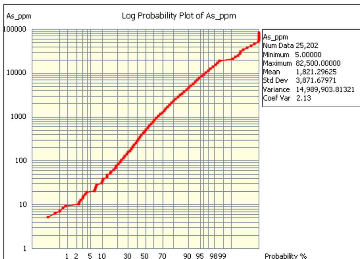
Figure 12: As (ppm) Log Probability Plot
