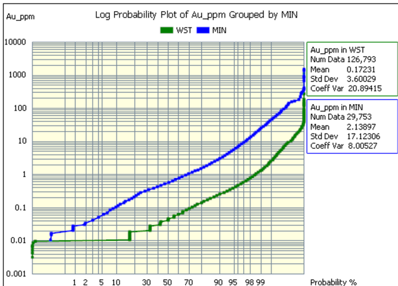
Figure 11: Au (g/t) Log Probability Plot
