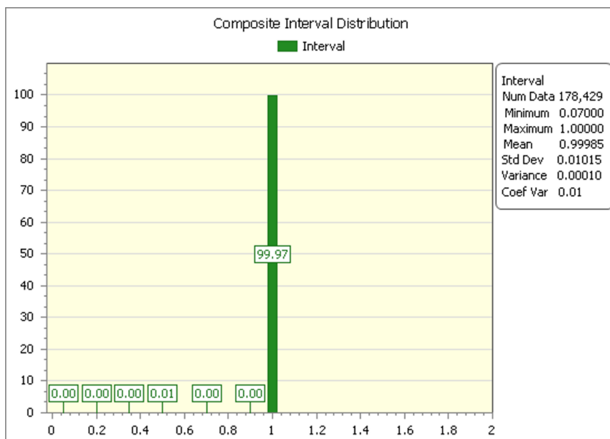
Figure 8: One Metre Composite Length Distribution
