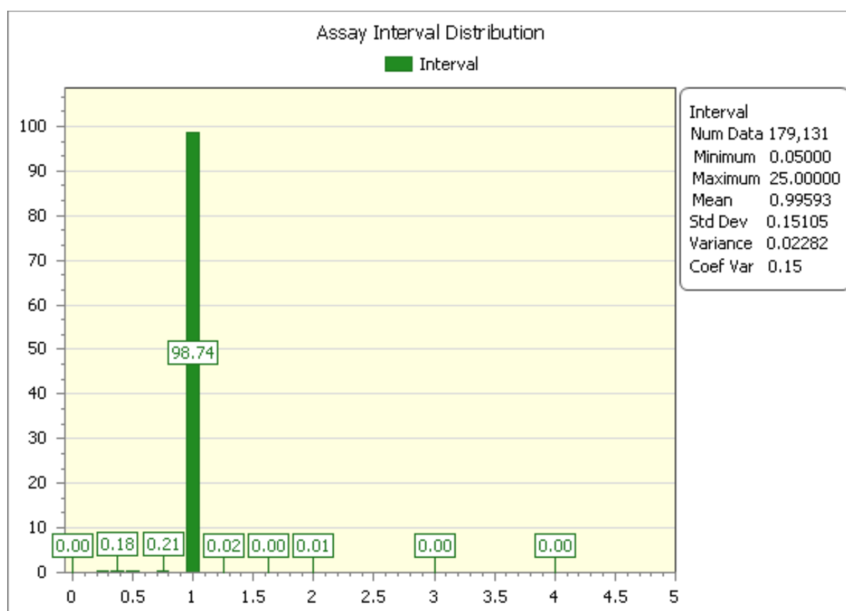
Figure 7: Assay Sample Length Distribution
