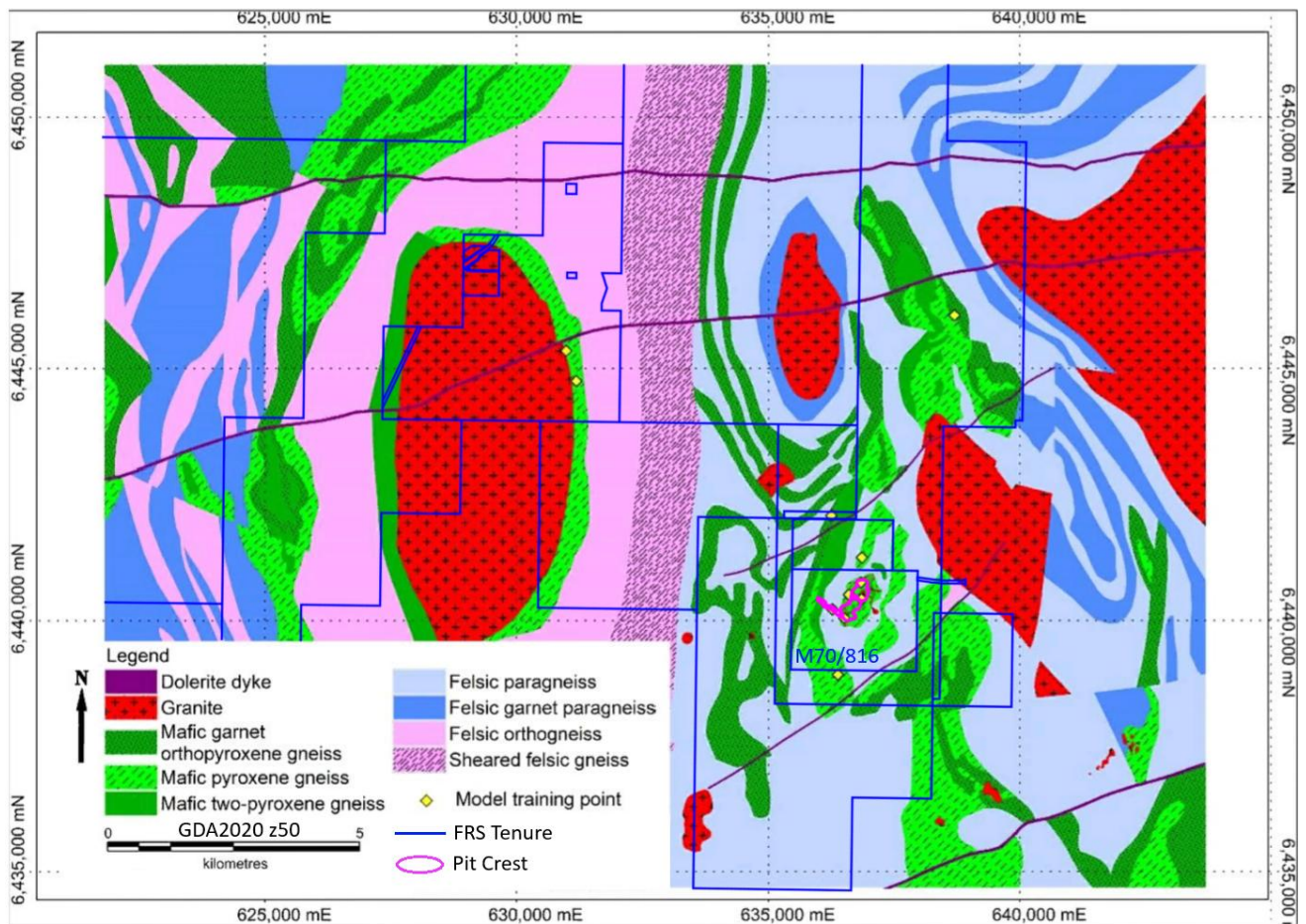
Figure 4: Project Geology with FRS Tenure and Pit Location
