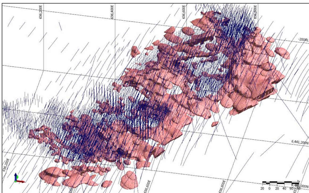
Figure 9: Perspective View of Implicit Model Wireframes and Drilling Data
