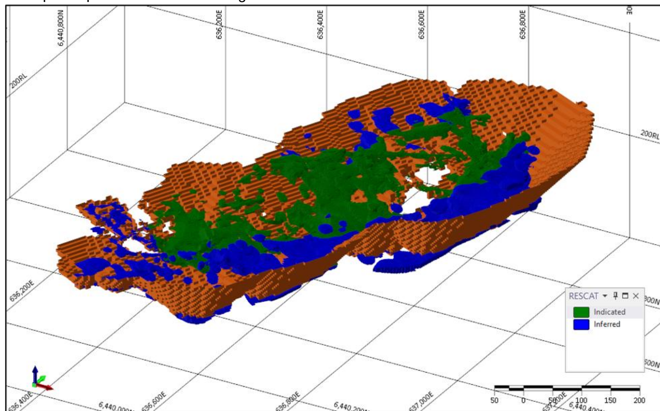
Figure 16: Tampia Deposit with AUD 6,000 Optimal Pit Shell
