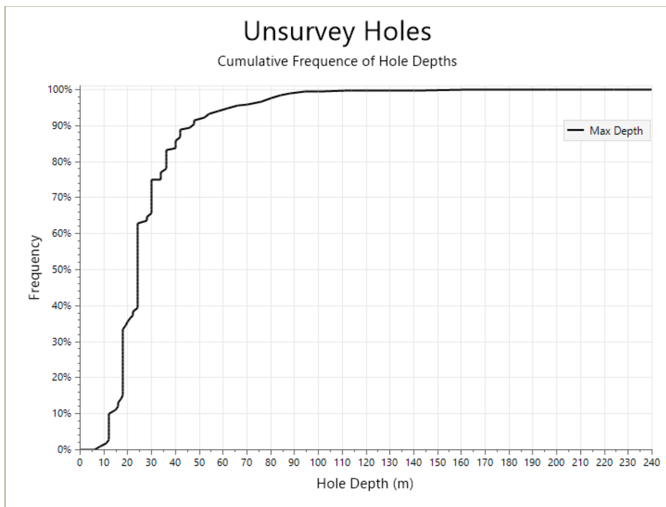
Figure 6: Cumulative Frequency Plot of the Maximum Depth of Unserved Drill Holes
