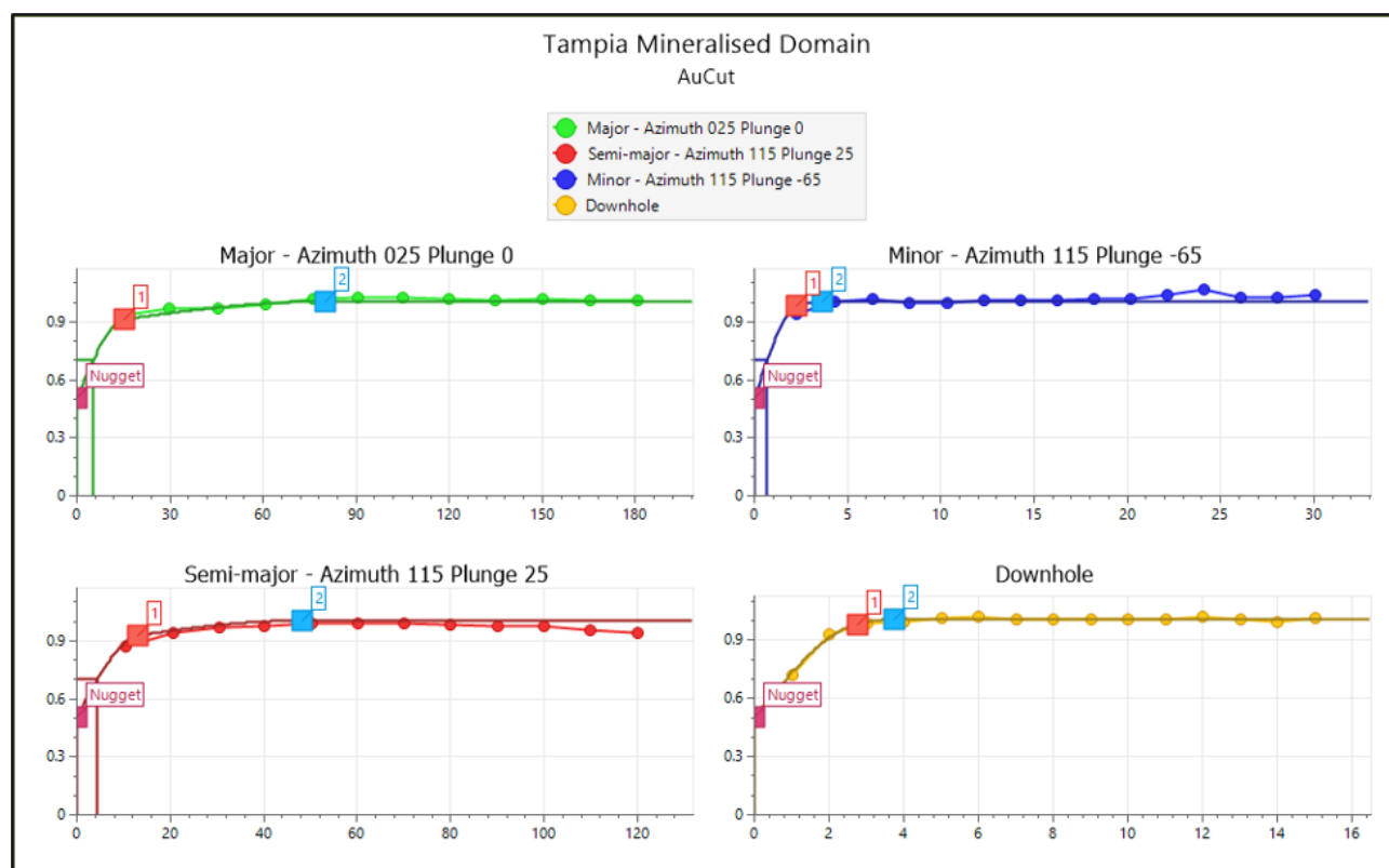
Figure 14: Variogram Models
