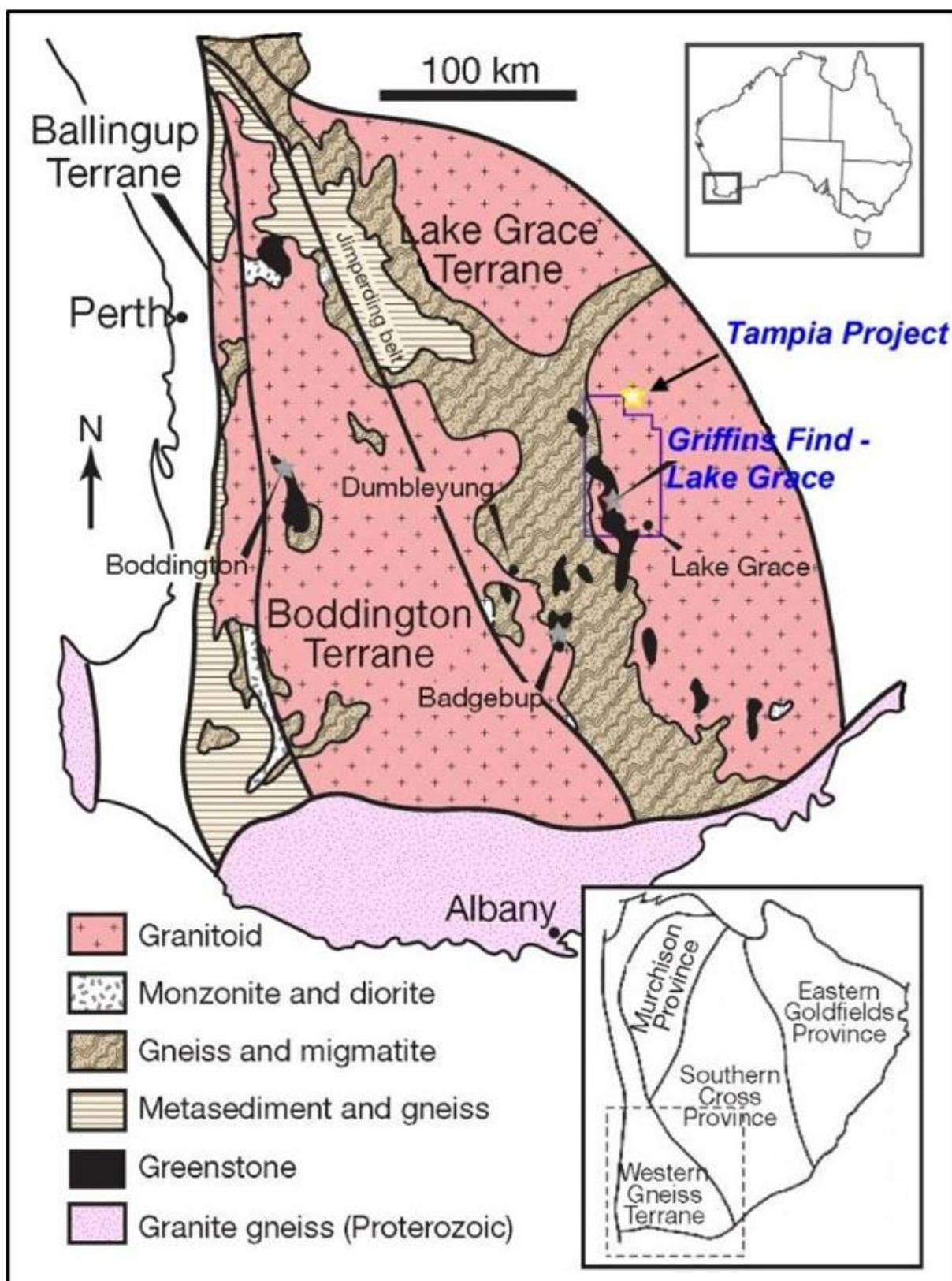
Figure 3: Regional Geology of south-western Western Australia
