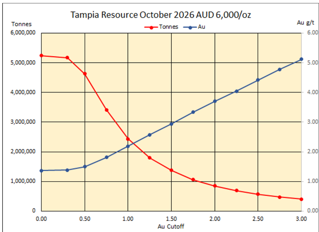
Figure 17: Optimal Grade Tonnage Curve for the Tampia Deposit (Indicated + Inferred)
