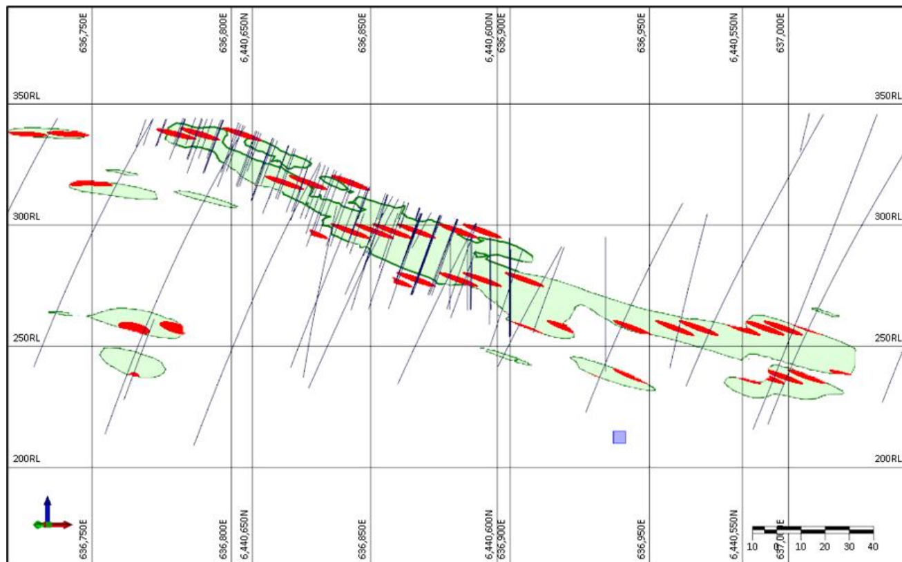
Figure 10: Variable Search Ellipse Orientations
