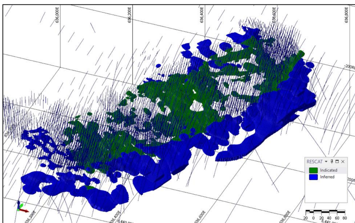
Figure 15: Resource Classification
