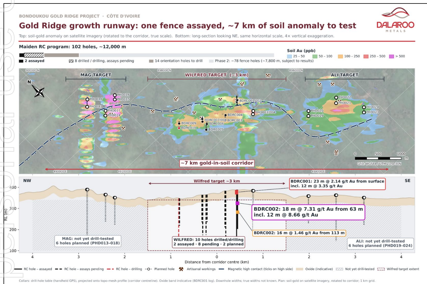
Figure 4. Mag, Wilfred and Ali targets along the ~7 km gold-in-soil corridor. Upper: soil-gold anomaly on satellite imagery with drill collars, planned holes, artisanal workings and interpreted magnetic contact. Lower: long-section looking north-east (4x vertical exaggeration) with Wilfred RC holes, planned Mag and Ali holes, and BDRC001 and BDRC002 intercepts. Downhole widths; true widths not known. Grid: WGS84 / UTM Zone 30N.
