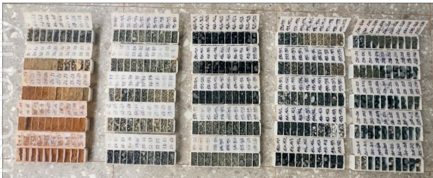
Figure 2. Chip trays of BDRC001.
