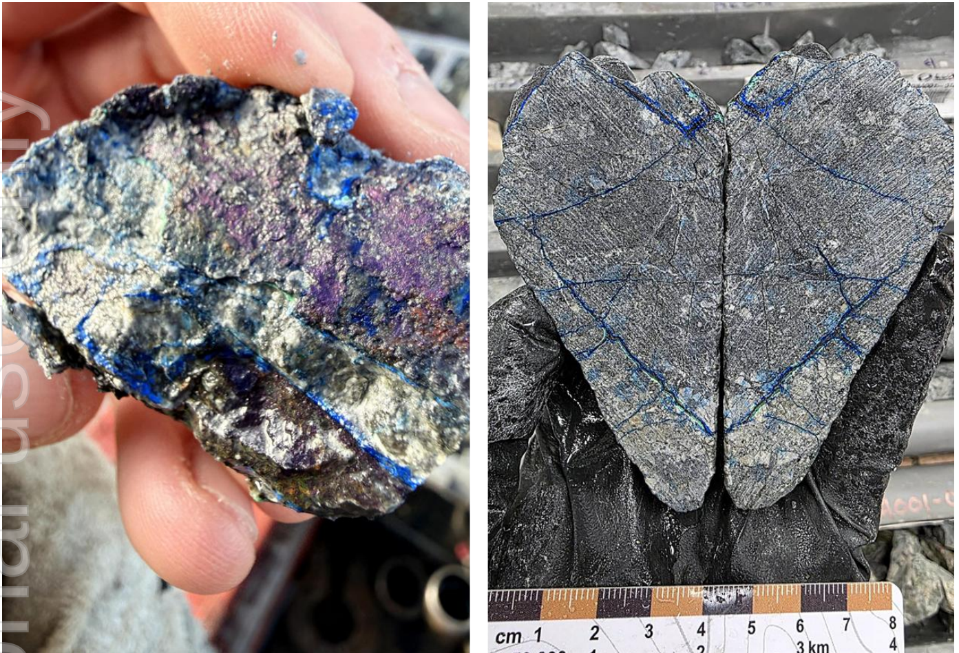
Figure 1: DDBA26-001 at 23.9m down-hole. Examples of copper-bearing mineralisation intersected at the Baird Project. Together, these samples demonstrate both the vibrant oxidation textures and the vein-style copper enrichment typical of near-surface and structurally influenced copper systems. LEFT – metallic, iridescent surface with vivid blue, purple, and silver tones characteristic of oxidized copper sulphides, bornite and chalcopyrite. RIGHT – a split core section with chalcocite veinlets and bright blue azurite vein margins cutting through a fine-grained dolomite.
