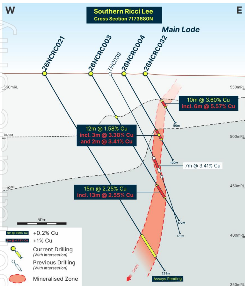
Figure 3: Ricci Lee Drill section 7173680N.
