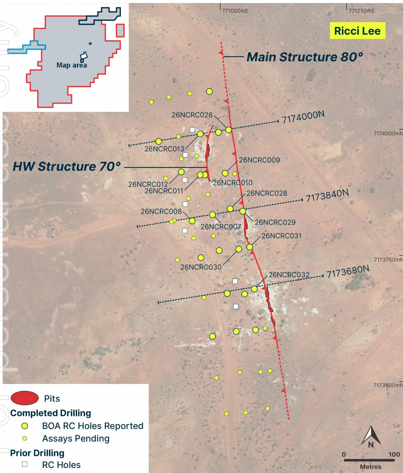
Figure 5: Ricci Lee Drill Plan.
