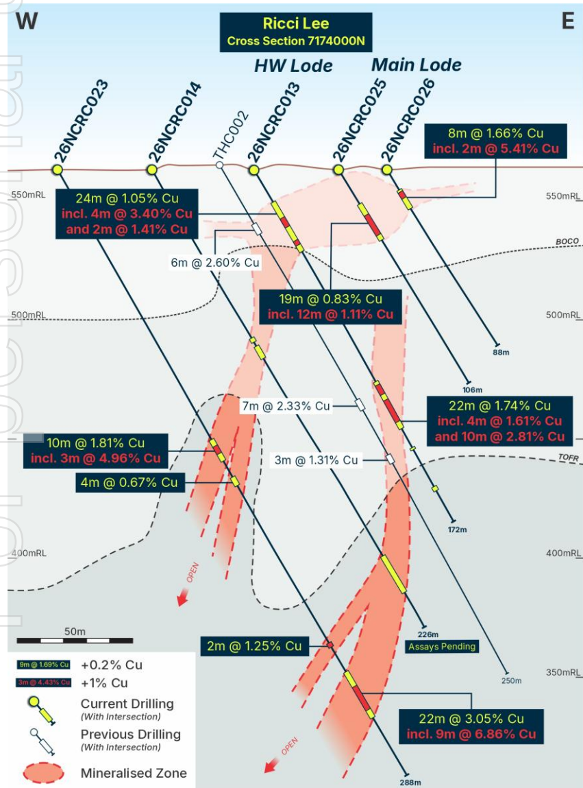
Figure 1: Ricci Lee Drill section 7174000N.
