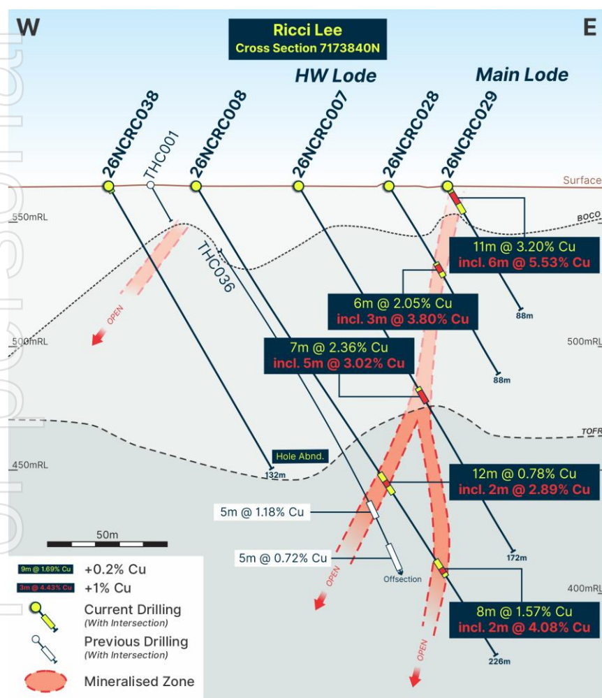
Figure 2: Ricci Lee Drill section 7173840N.
