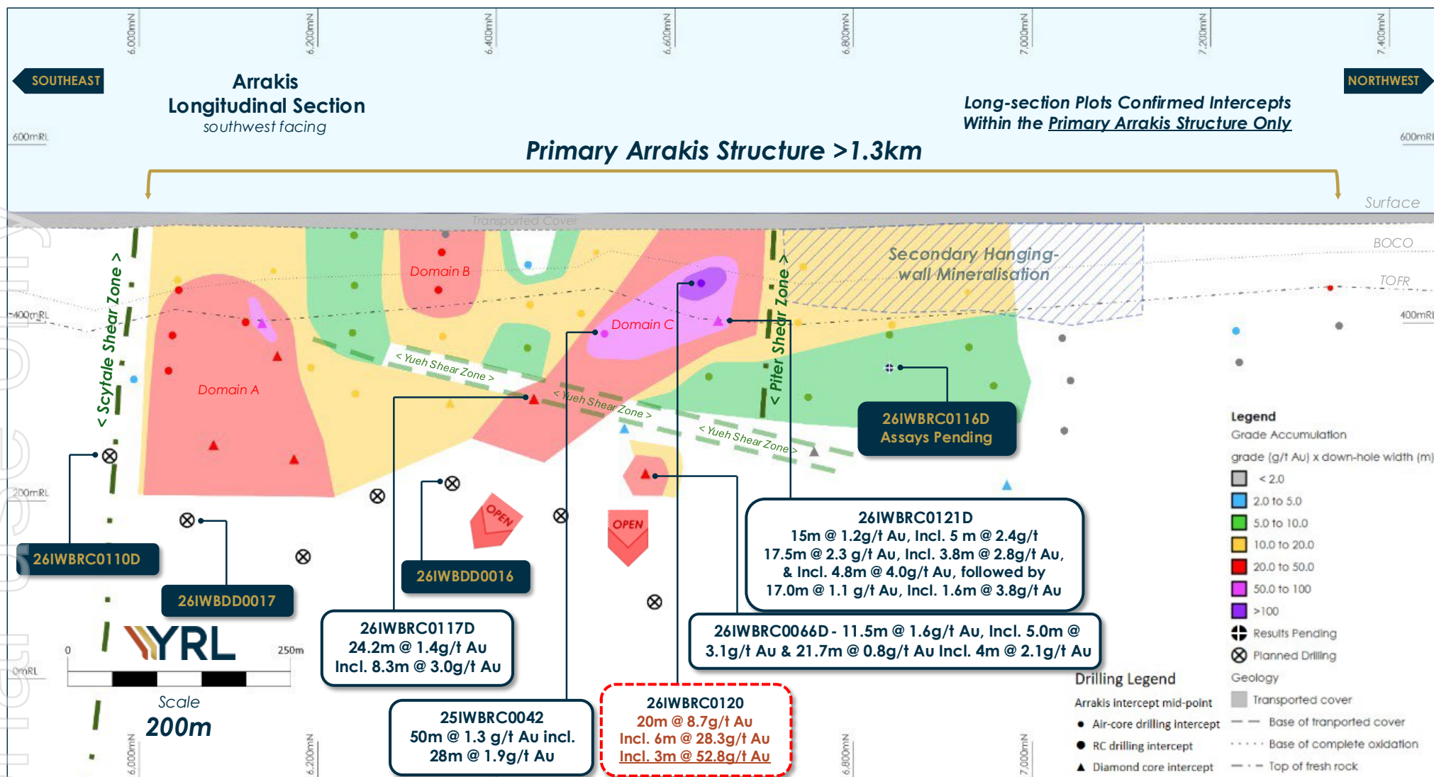
Figure : A longitudinal section displaying intercept midpoints within the main Arrakis mineralised structure (intercepts from subordinate structures are excluded). Grade accumulation (length multiplied by Au grade) is based on down-hole length, with no true width correction applied. This longitudinal section has been prepared to show the distribution of recent intercepts across the interpreted Arrakis trend. Contours are based on grade (g/t Au) multiplied by down-hole length (m) values, and are presented to provide a visual interpretation of high-grade domains across the Arrakis mineralised system. Please note that closer-spaced drilling is needed to verify geological and grade continuity along strike. Closer-spaced drilling is also needed to verify the geometry and extent of the higher-grade domains contoured in this longitudinal section.
