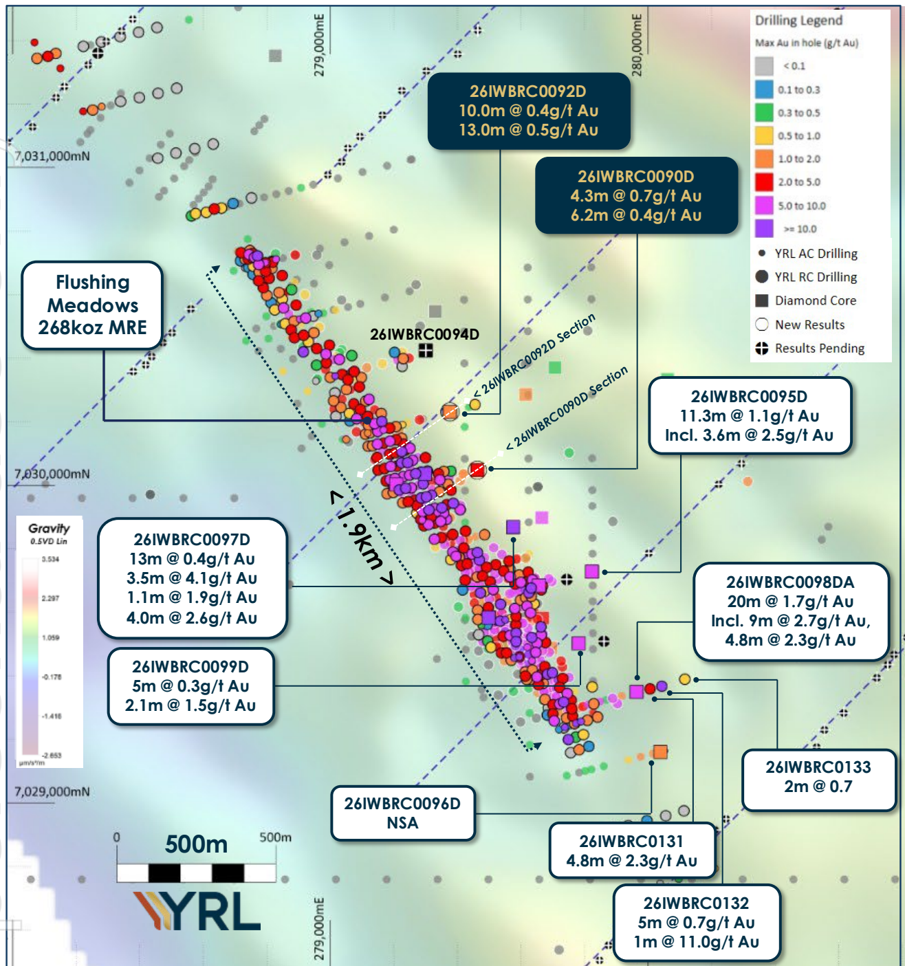
Figure 6: Flushing Meadows collar plan overlaid on a ground gravity image (BA267 0.5VD non-linear colour scale, with northeast shading). All Yandal drilling is plotted, with only effective (>20m down-hole depth) historic drilling displayed. Collars are thematically coloured by max Au (g/t) in the hole. The section lines for Figures 4 and 5 are also displayed. The diagram shows that previous drilling has been very ineffective around the current MRE, particularly to the east and southeast.
