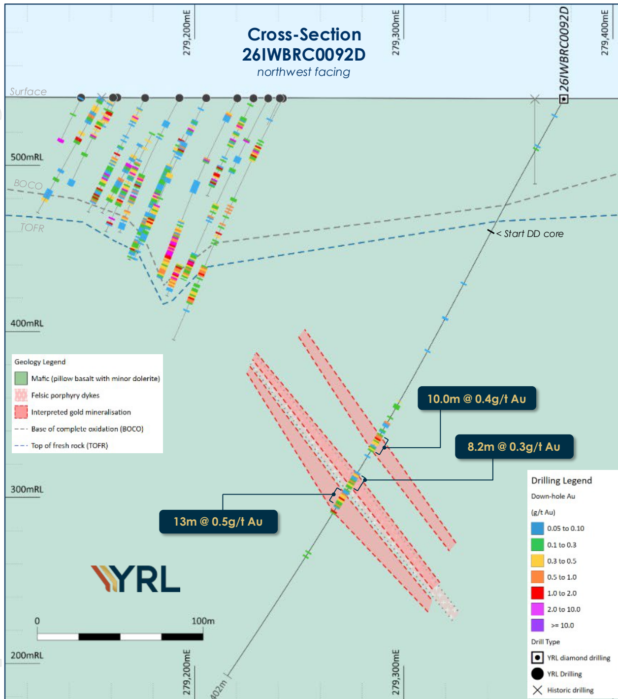
Figure 5: Cross-section showing mineralised intervals from 261WBRC0092D at Flushing Meadows. The section location is shown in Figure 6. The section shows all drilling within +/- 25m of the section plane.
