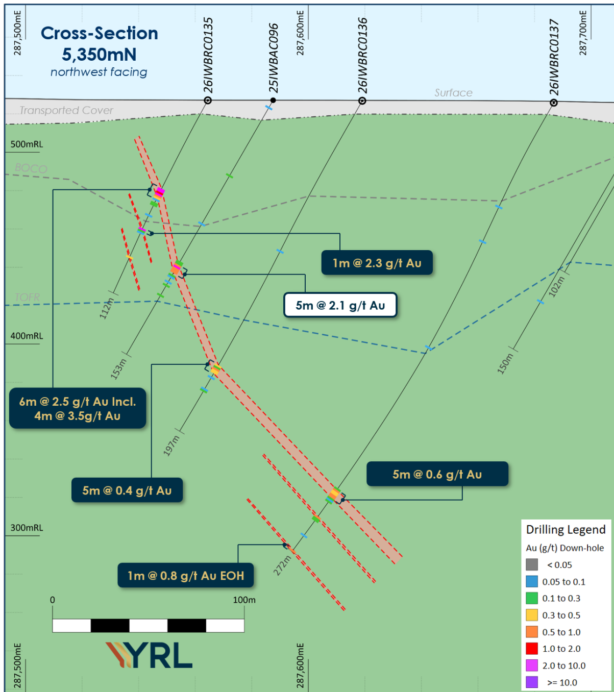
Figure 3: Cross-section showing mineralised intervals from 26IWBRC0135, 26IWBRC0136 and 26IWBRC0137 from the Anders Prospect. The section location is shown in Figure 2. The section shows all drilling within +/- 25m of the section plane.
