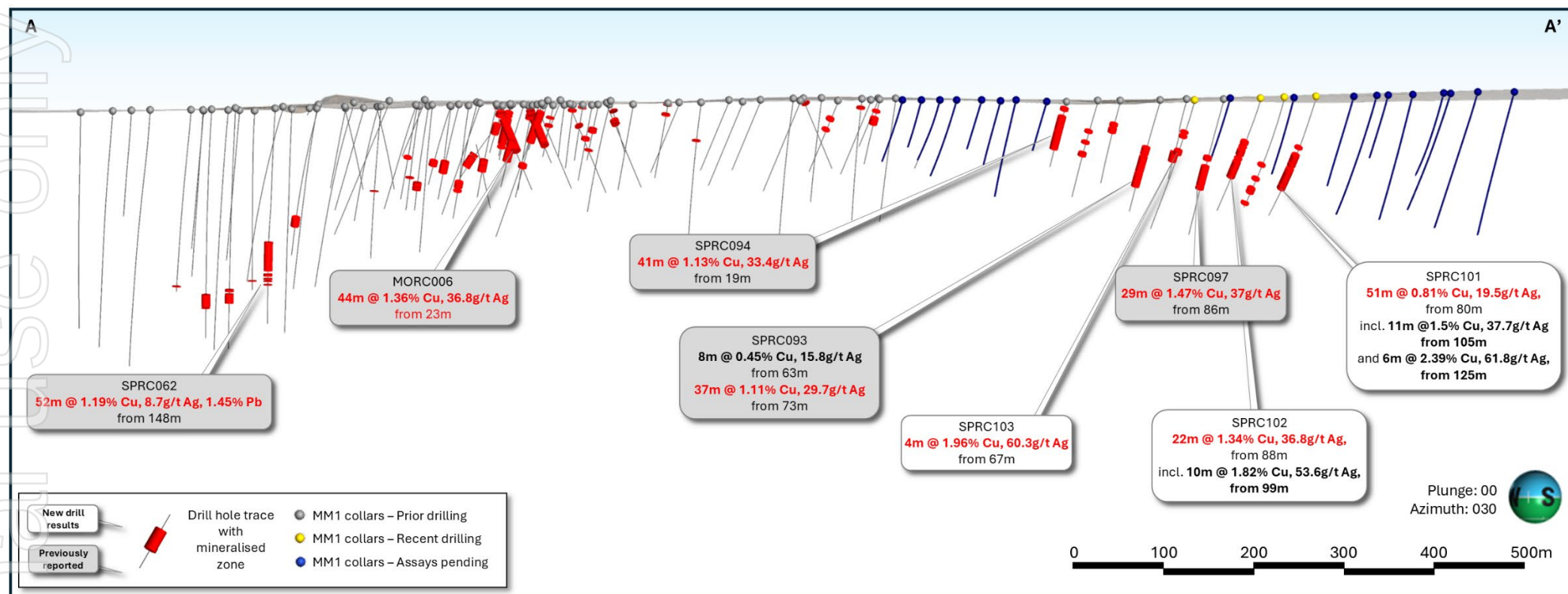
Figure 2: Oblique cross section (A-A') of Spaatzu Deposit looking North Eastly (refer Figure 1). 1,2
