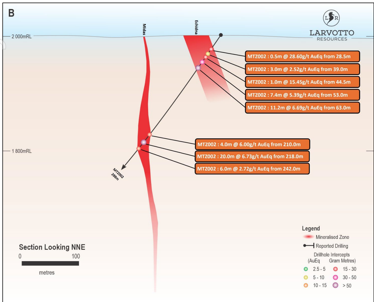
Figure 4: Midas Section B–B', extending from surface to more than 450 m below surface through drill hole MTZ002, highlighting significant Midas drill intersections and the near-surface Echidna Lode, which strikes orthogonal to the Midas Lode.
