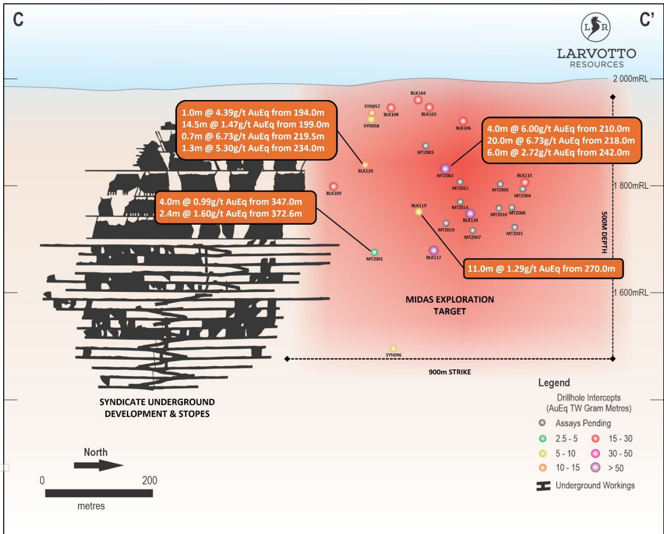
Figure 5: Syndicate and Midas Lode Long Section showing estimated true width (ETW) gram metres of reported and previously reported Midas Drill Intercepts.
