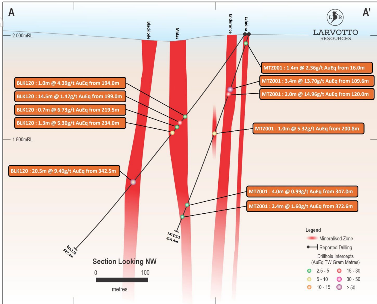
Figure 3: Blacklode-Midas-Endurance Section A-A', extending from surface to more than 450 m below surface through drill hole BLK120 and MTZ001, highlighting significant Blacklode, Midas, Endurance and Echidna drill intersections
