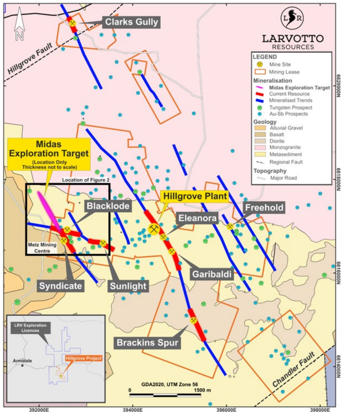
Figure 1 Hillgrove Project location, showing the Metz Mining Centre relative to the Hillgrove Plant, current resources, mineralised trends and gold-antimony-tungsten prospects.
