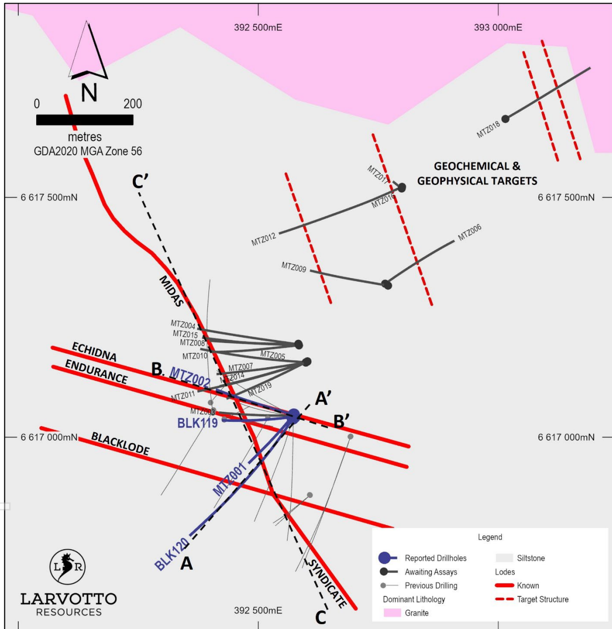
Figure 2: Metz Mining Centre showing the Blacklode, Midas, Endurance, Syndicate and Echidna lodes, the location of reported drill holes and the location of drill sections displayed below
