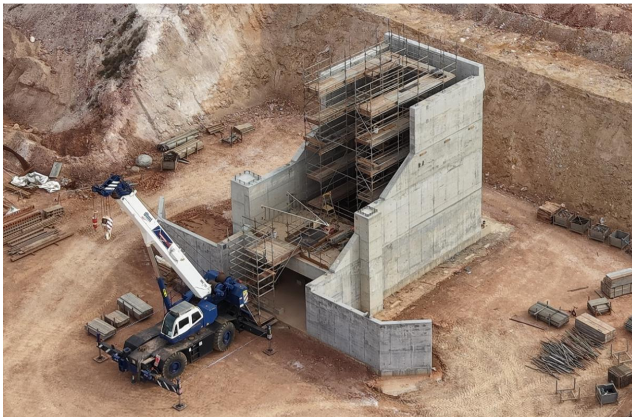
Figure 2 – Primary Crusher – final pour completed
