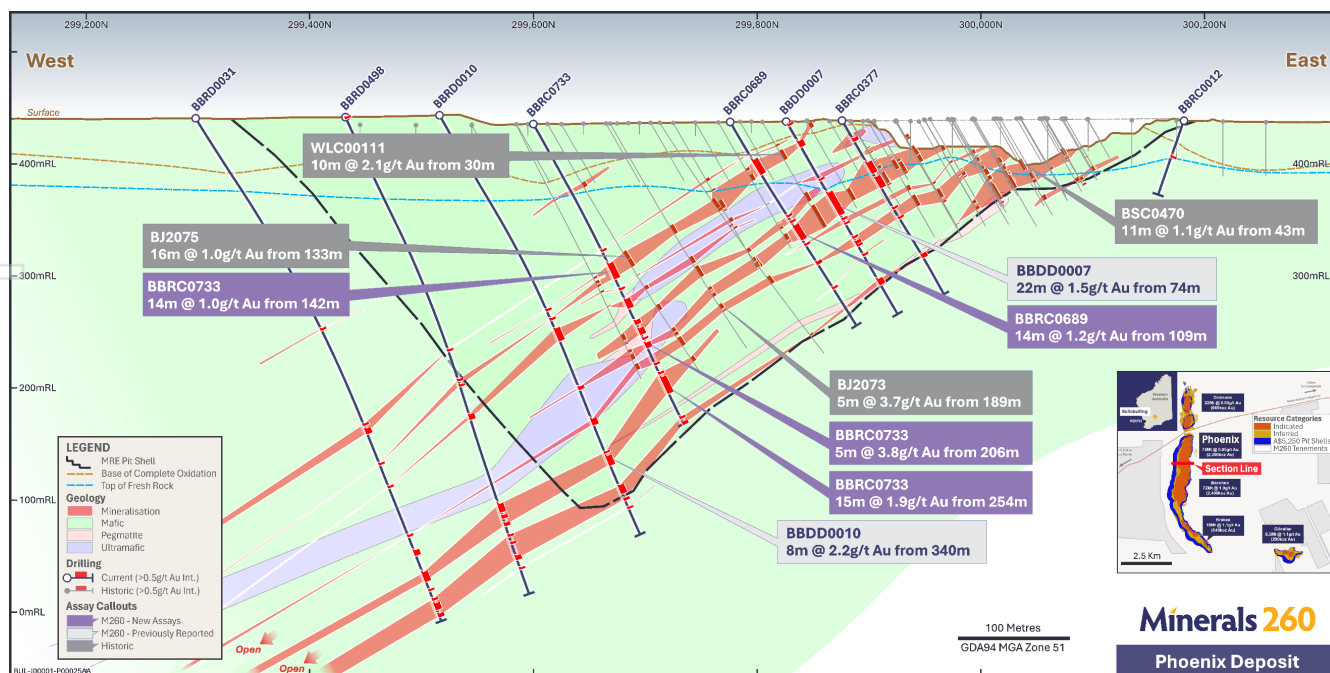
Figure 2: Section 6567680N showing mineralisation in BBRC0689 and BBRC0733 infilling Phoenix MRE pit shell (new results in purple boxes)
