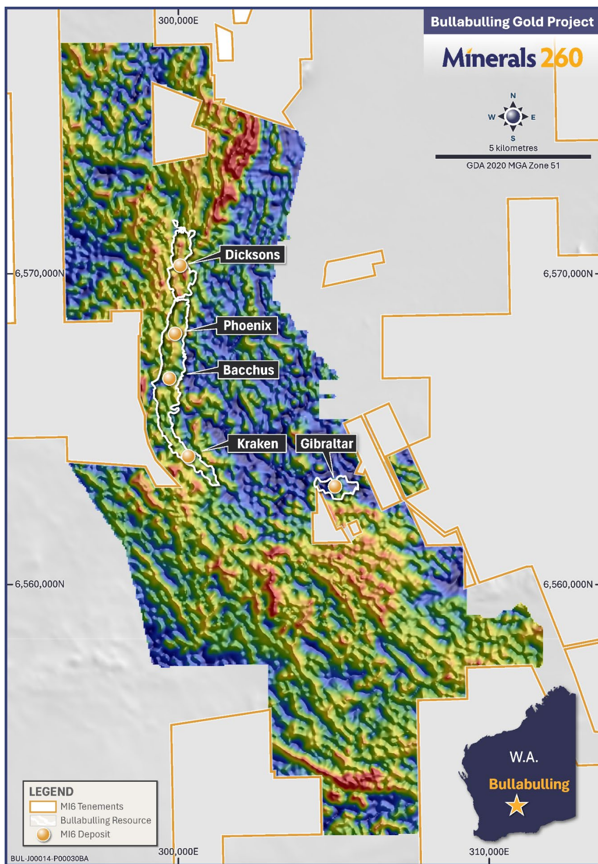
Figure 5: Regional ground gravity survey with MRE footprint (red – gravity high, blue – gravity low)
