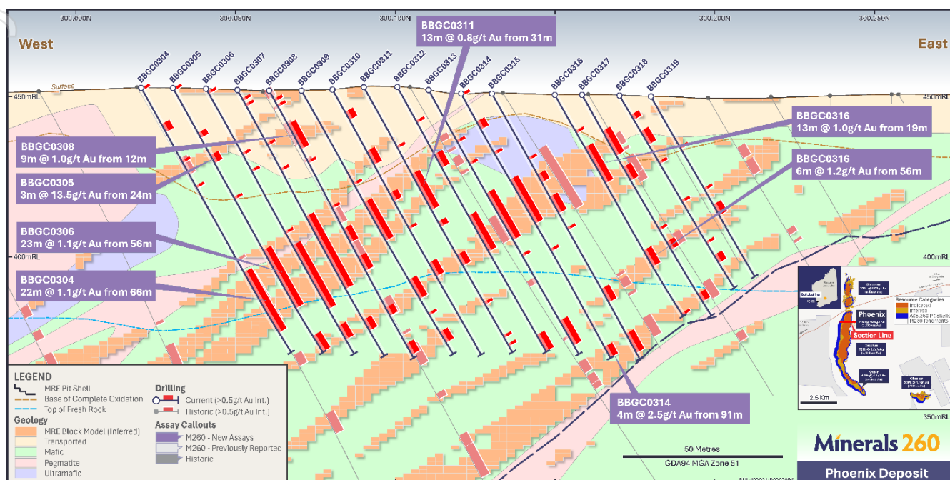
Figure 1: Section 6568350N showing mineralisation in grade control drilling testing the Phoenix MRE pit shell (new results in purple boxes)
