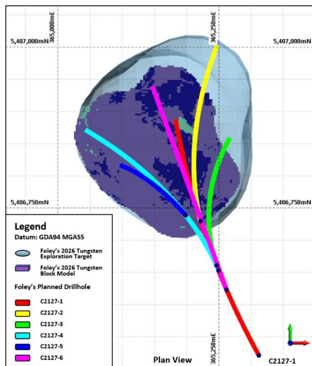
Figure 2. Plan view of the planned diamond drilling target at Cleveland
