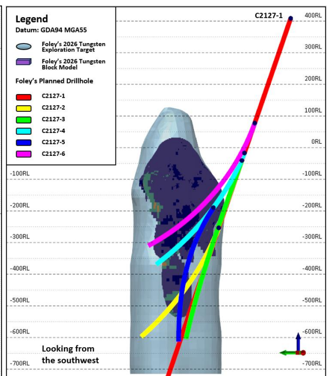
Figure 3. Section looking from the southwest of the planned diamond drilling target
