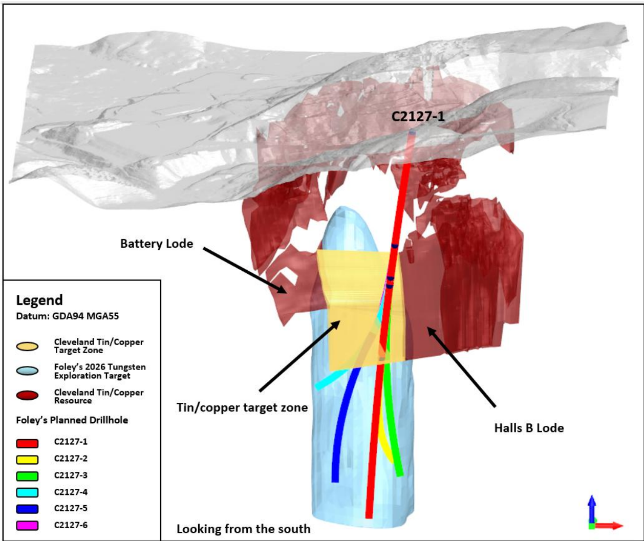
Figure 1. View looking north (from the south) of the planned drilling into the prospective tin/copper stratigraphy between the Halls B Lode and Battery Lode, that has not been drill tested by historical drilling campaigns.
