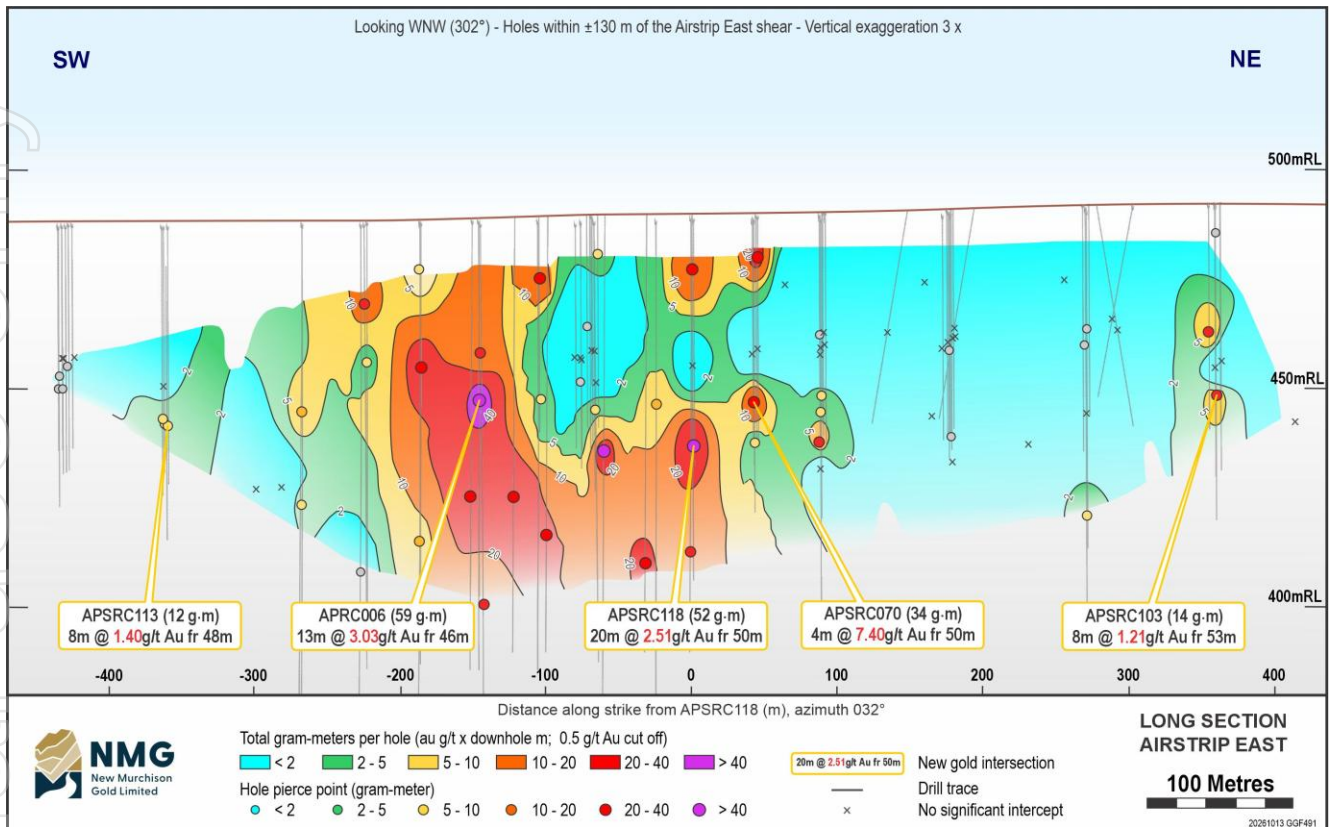
Figure 4: Airstrip East long section contoured by gram-metres (grade × downhole width) per hole
