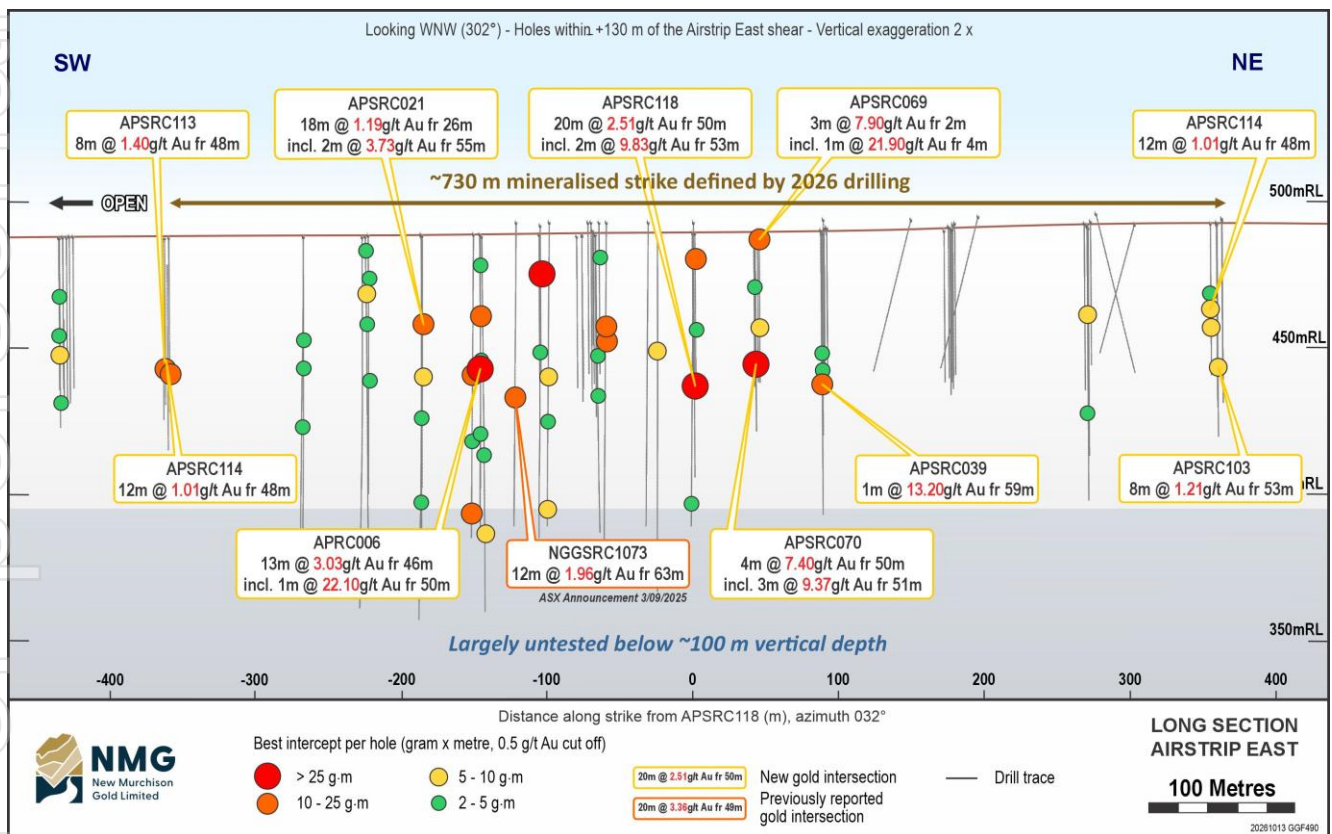
Figure 3: Airstrip East longitudinal section showing intercept pierce points and ~730m of mineralised strike
