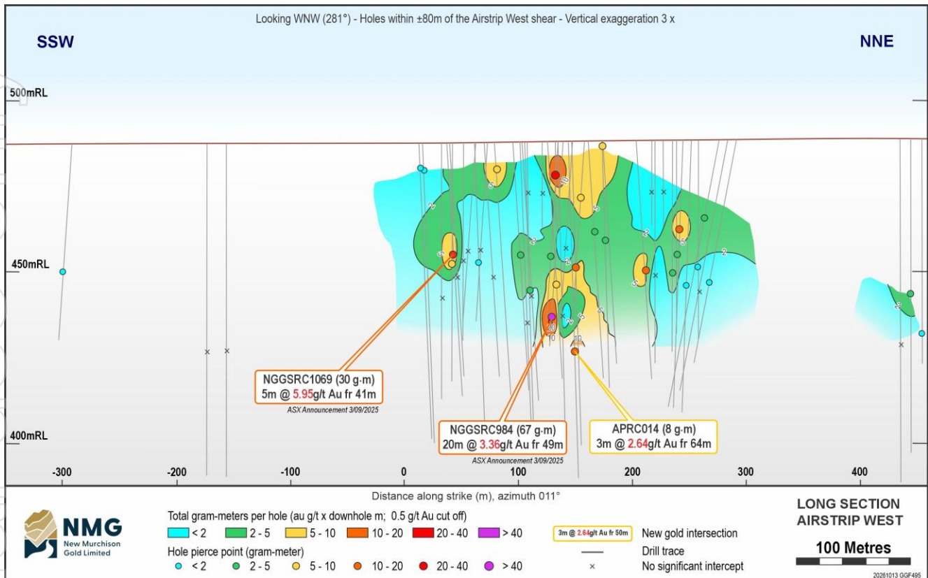
Figure 8: Airstrip West long section contoured by gram-metres per hole
