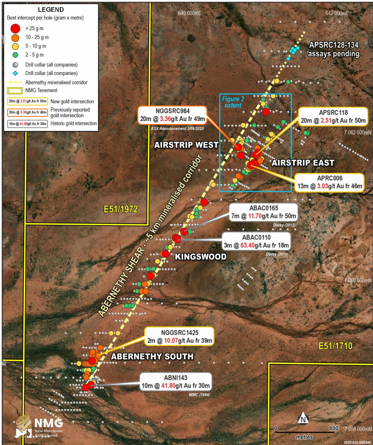
Figure 9: Abernethy Shear corridor – regional drilling plan showing best intercept per hole on aerial imagery
