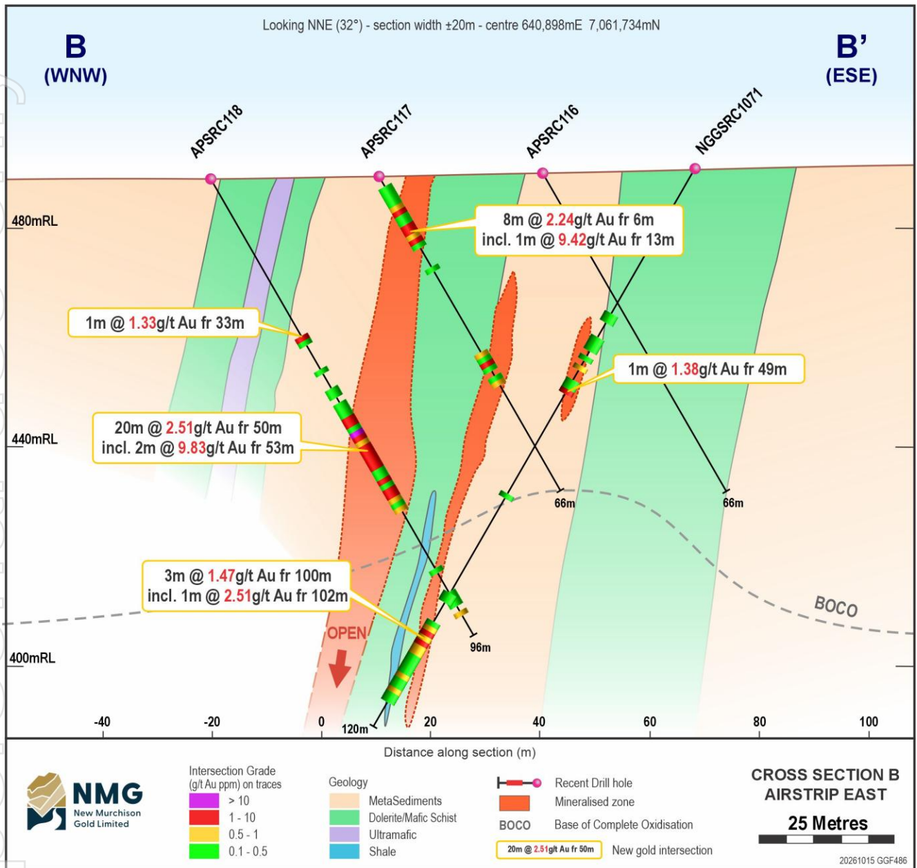
Figure 6: Cross section B-B' through APSRC11
