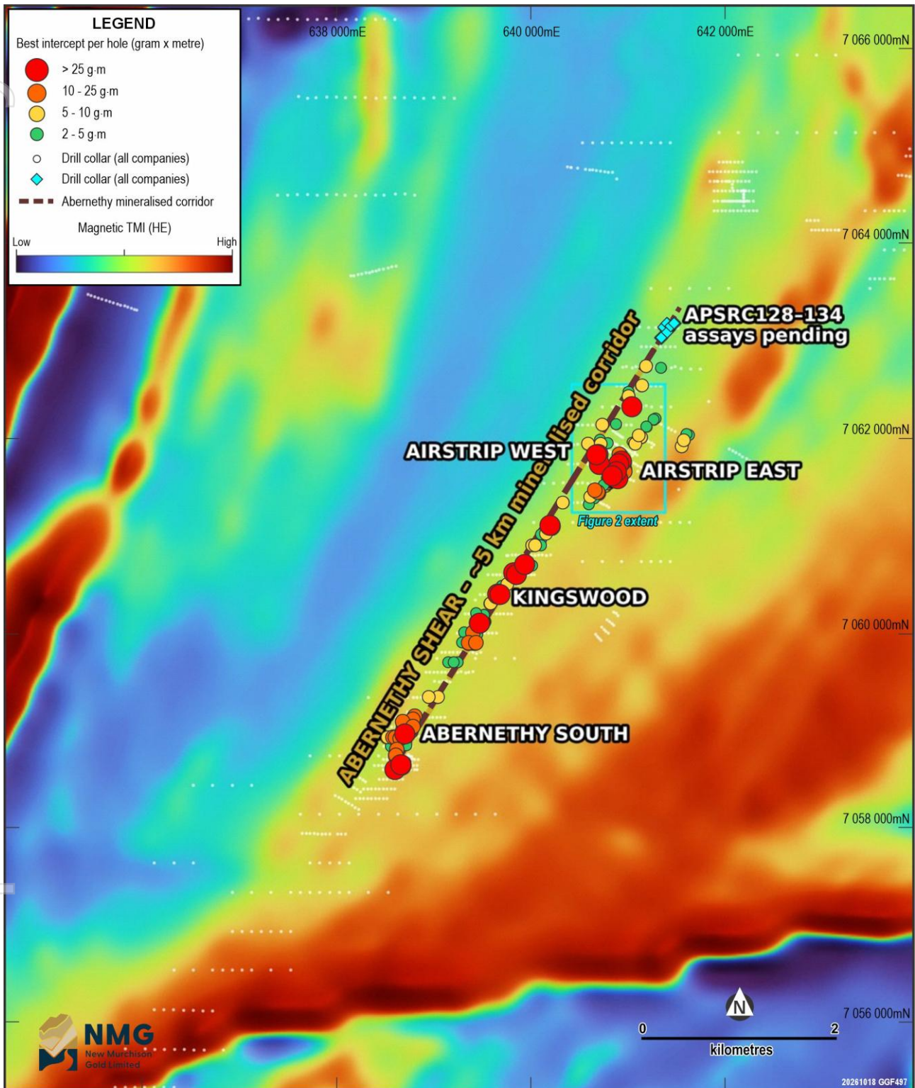
Figure 10: Abernethy Shear corridor on regional total magnetic intensity (Geoscience Australia 2019, 40m grid)
