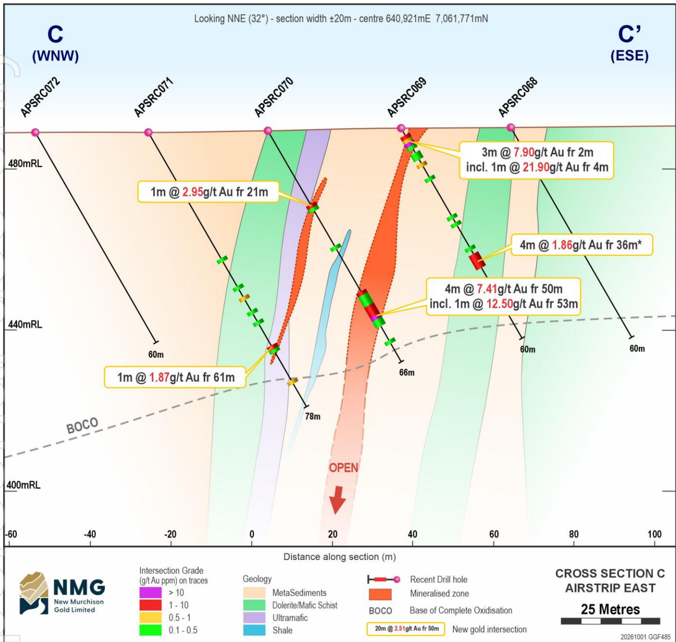
Figure 7: Cross section C–C' through APSRC070
