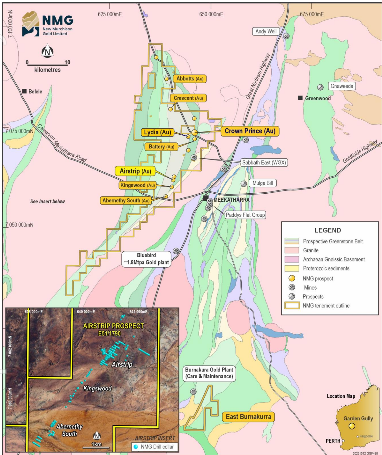
Figure 1: Location of the Airstrip prospect and Abernethy Shear corridor within the Garden Gully Gold Project
