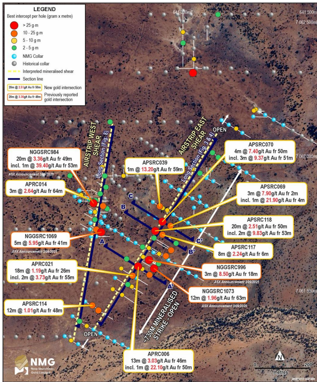
Figure 2: Airstrip prospect drill collar plan showing best intercept per hole, interpreted mineralised shears and cross-section locations
