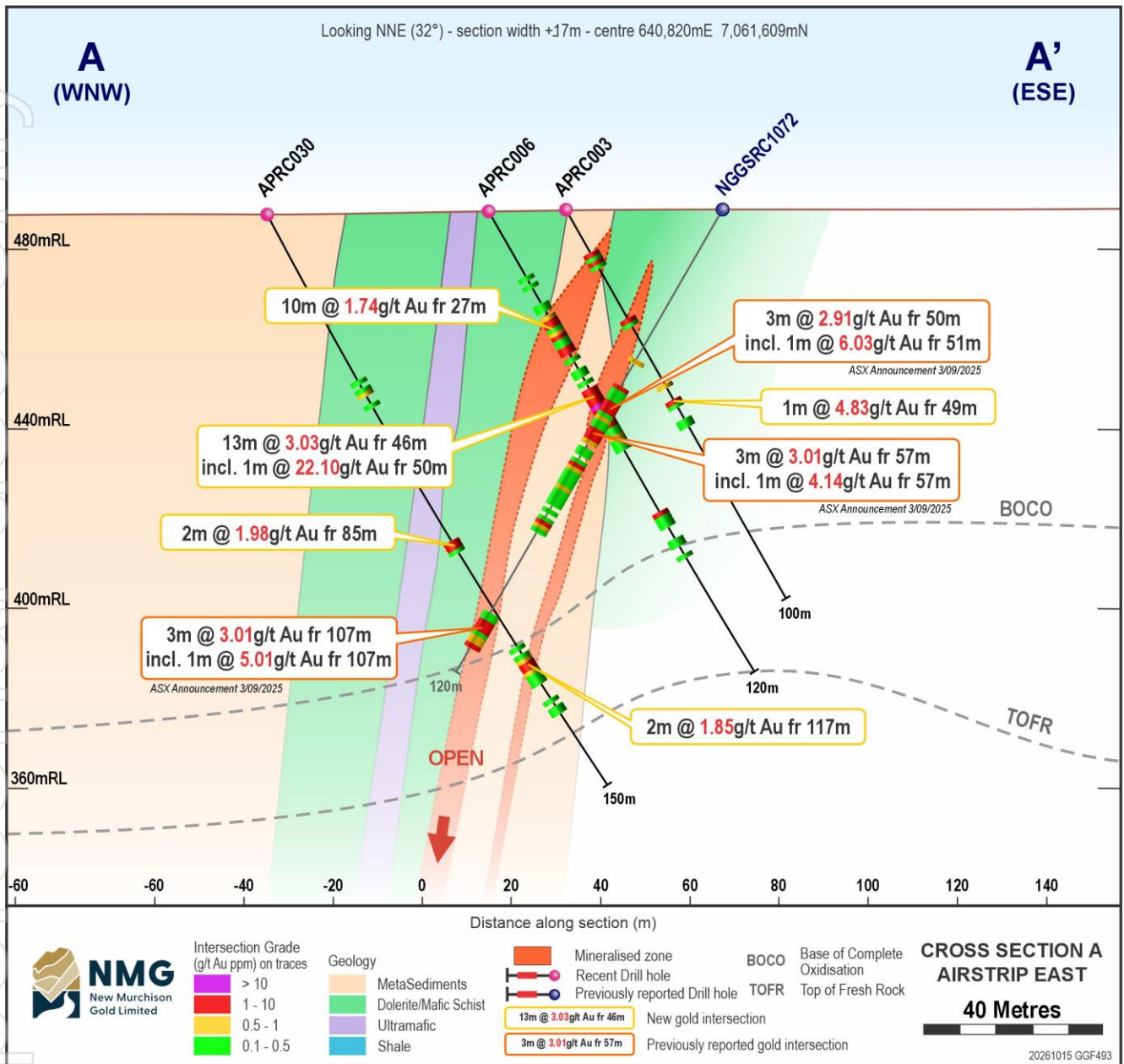
Figure 5: Cross section A–A' through APRC006
