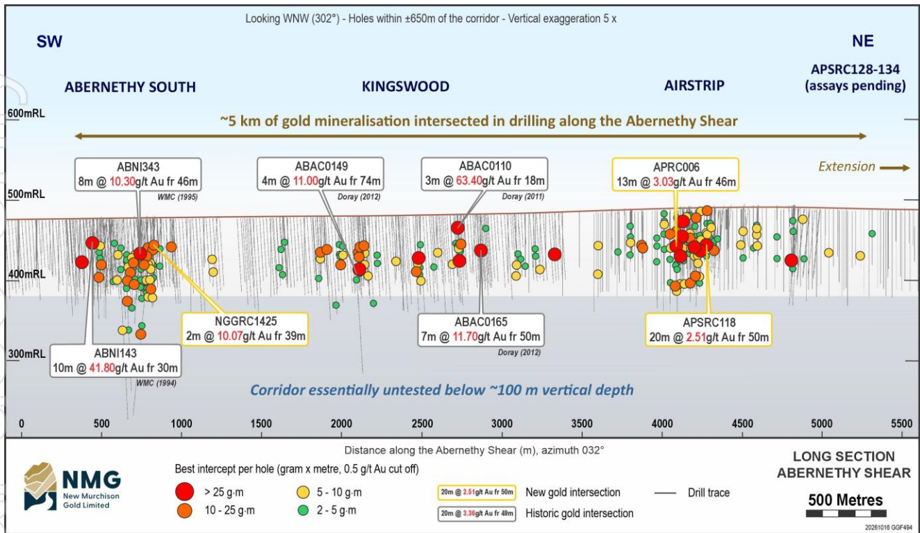
Figure 11: Abernethy Shear regional longitudinal section – Abernethy South to Airstrip
