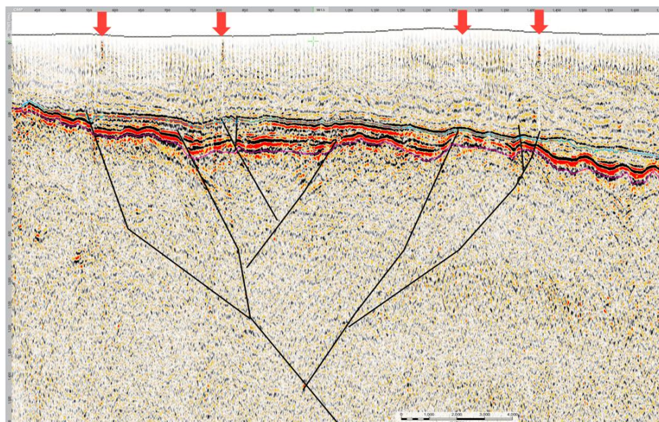
Figure 1: Seismic Line 84-TZJ over the Seabrook Lead, PELA 753. Red arrows show interpreted gas chimneys. Seismic data source: South Australian Resources Information Gateway. Government of South Australia, accessed 01/09/2026.
