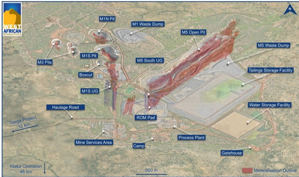
Sanbrado schematic layout
