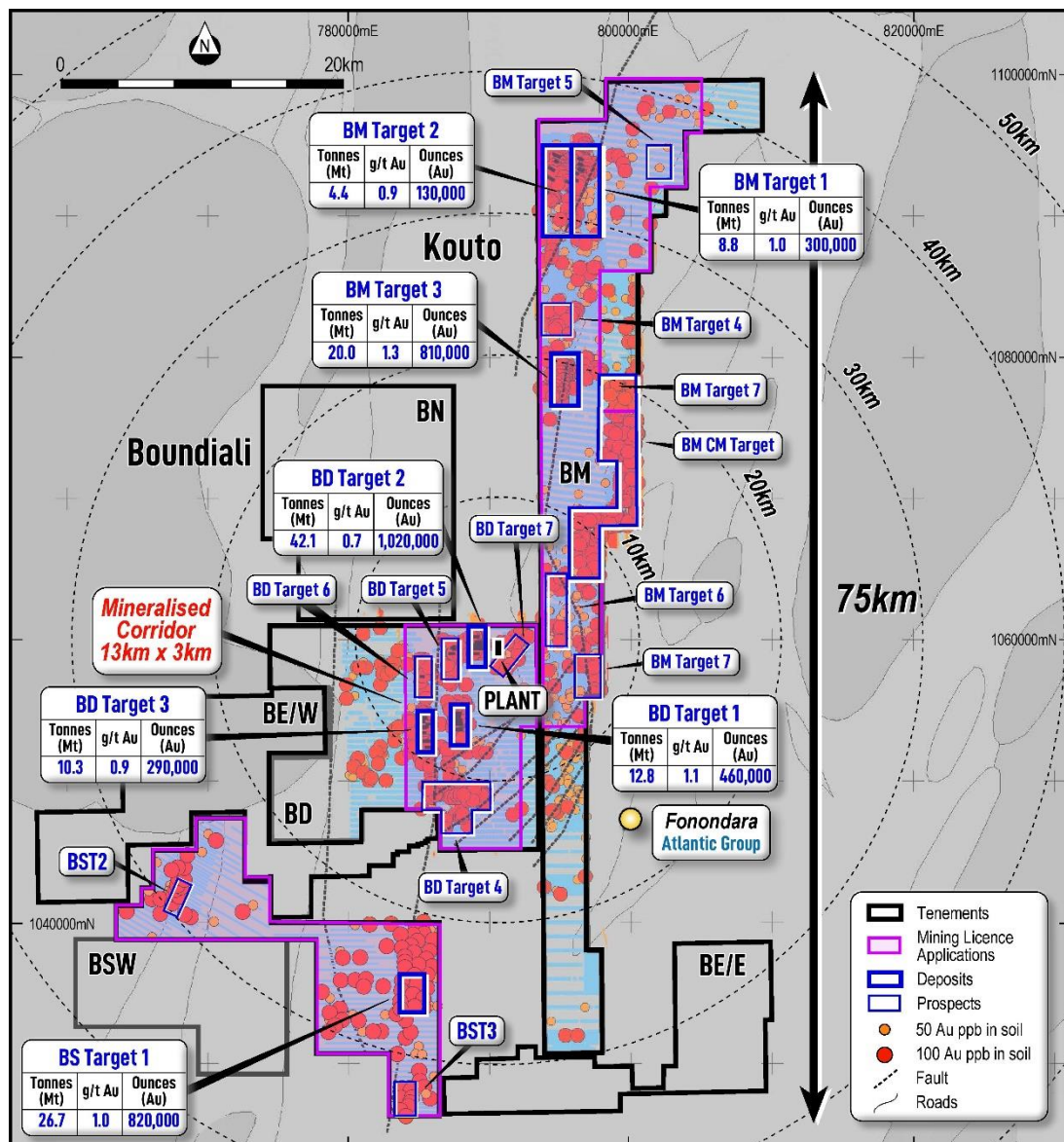
Figure 35: Plan View showing location of Boundiali Mineral Resources
