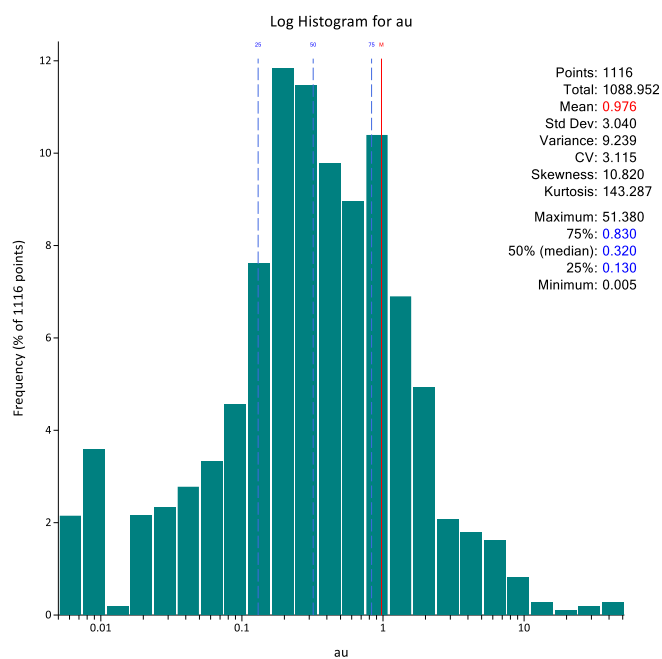
Figure 11: Log histogram for BMT2 composites (all)
