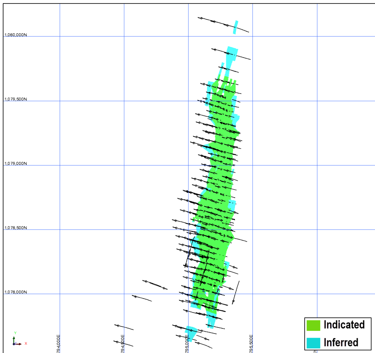
Figure 24: Plan view of BMT3 showing model classification (projected to surface with informing drilling)
