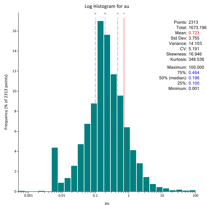
Figure 9: Log histogram for BDT3 composites (all)
