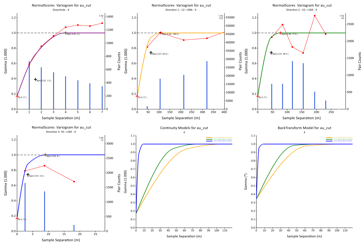
Figure 19: Experimental Variograms and fitted models BMT3 Object 4
