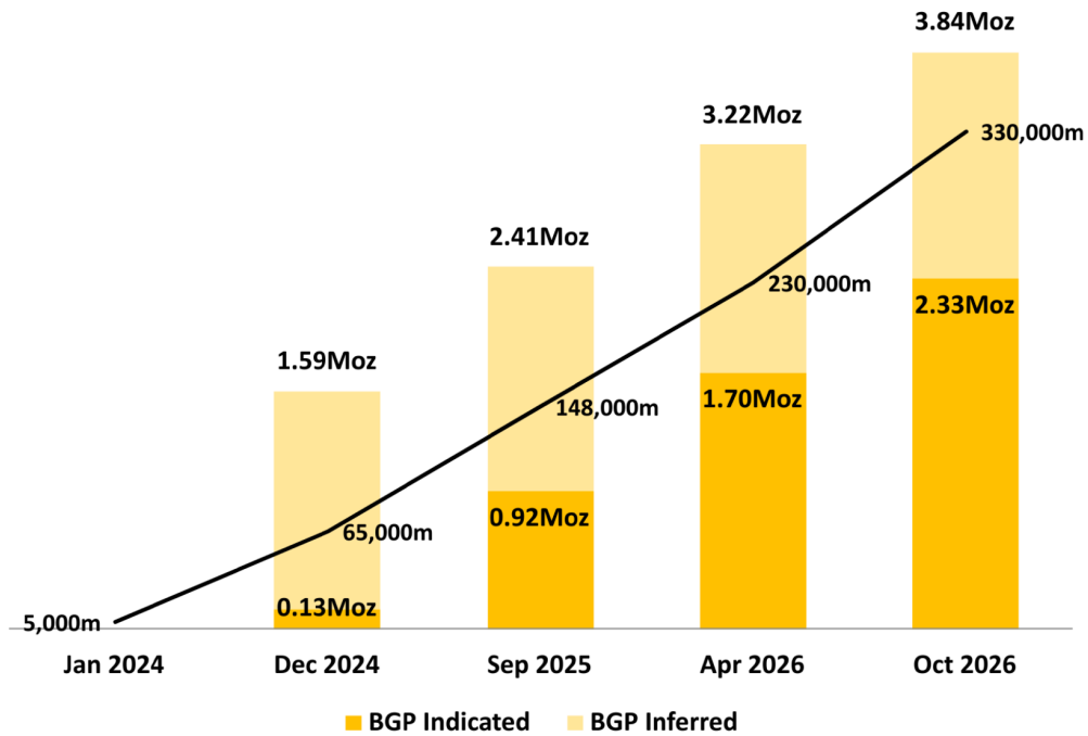
Figure 1: Boundiali Mineral Resource growth timeline
