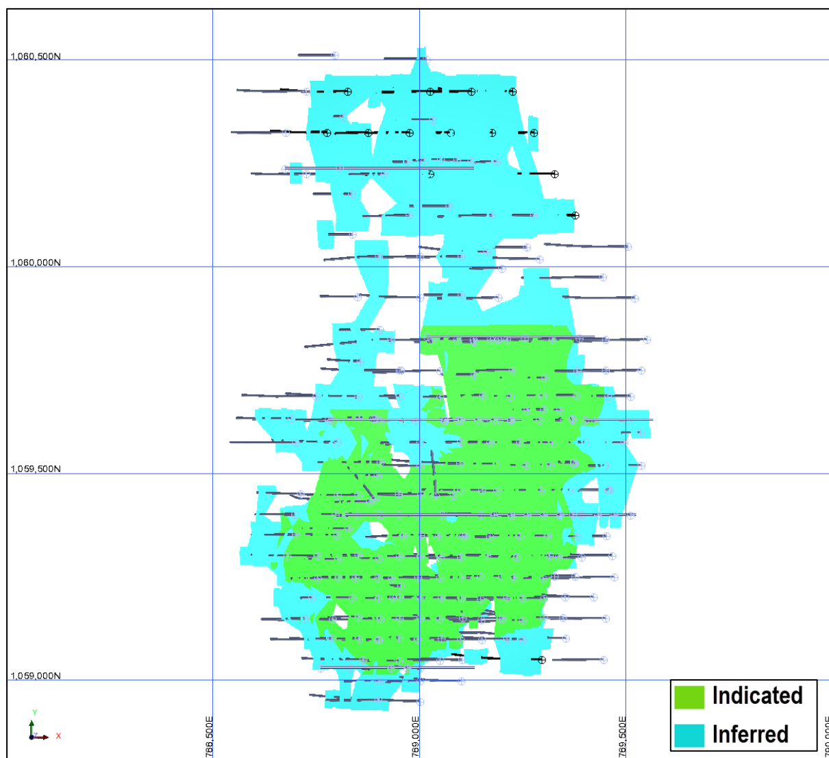
Figure 20: Plan view of BDT2 showing model classification (projected to surface with informing drilling)
