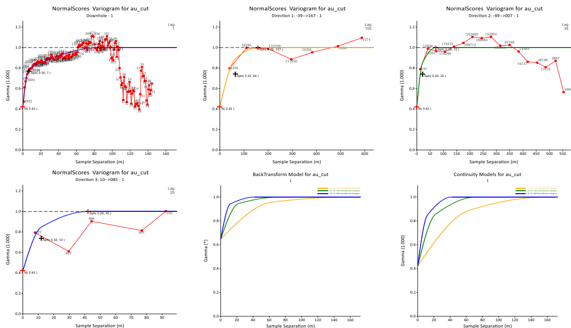
Figure 14: Experimental Variograms and fitted models BDT1 Object 1
