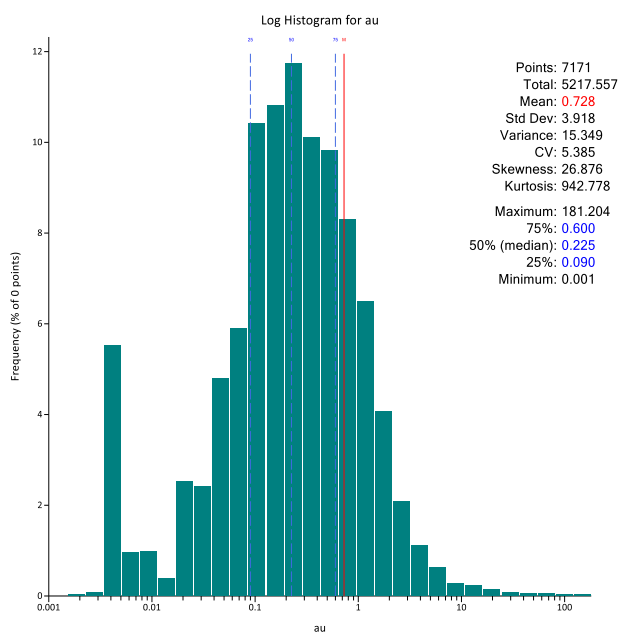
Figure 7: Log histogram for BDT1 composites (all)
