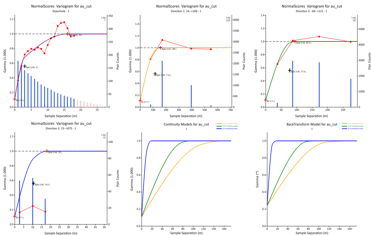
Figure 16: Experimental Variograms and fitted models BDT3 Object 1
