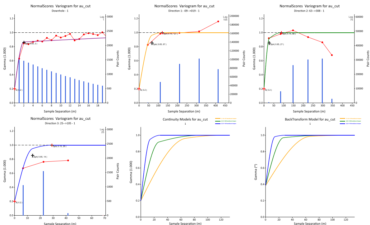
Figure 15: Experimental Variograms and fitted models BDT2 Object 1
