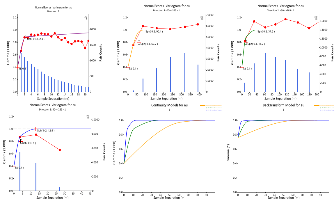
Figure 13: Experimental Variograms and fitted models BST1 Object 1
