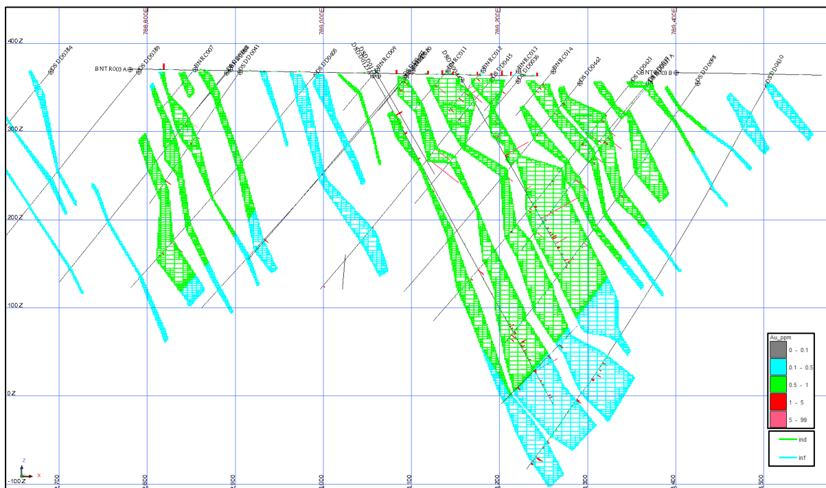
Figure 26: Example cross section (1,059,625mN) BDT2 showing resource classification and drill data (looking north +/-25m)
