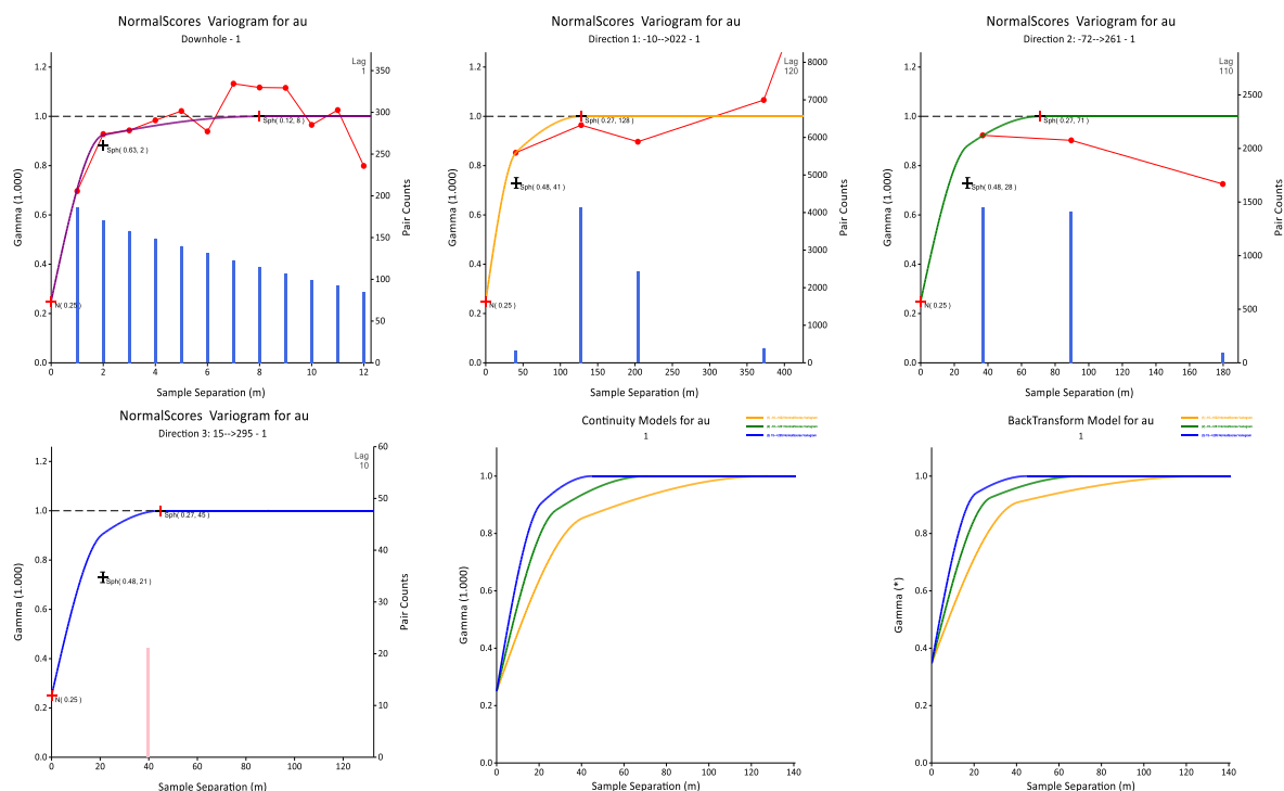
Figure 18: Experimental Variograms and fitted models BMT2 Object 1
