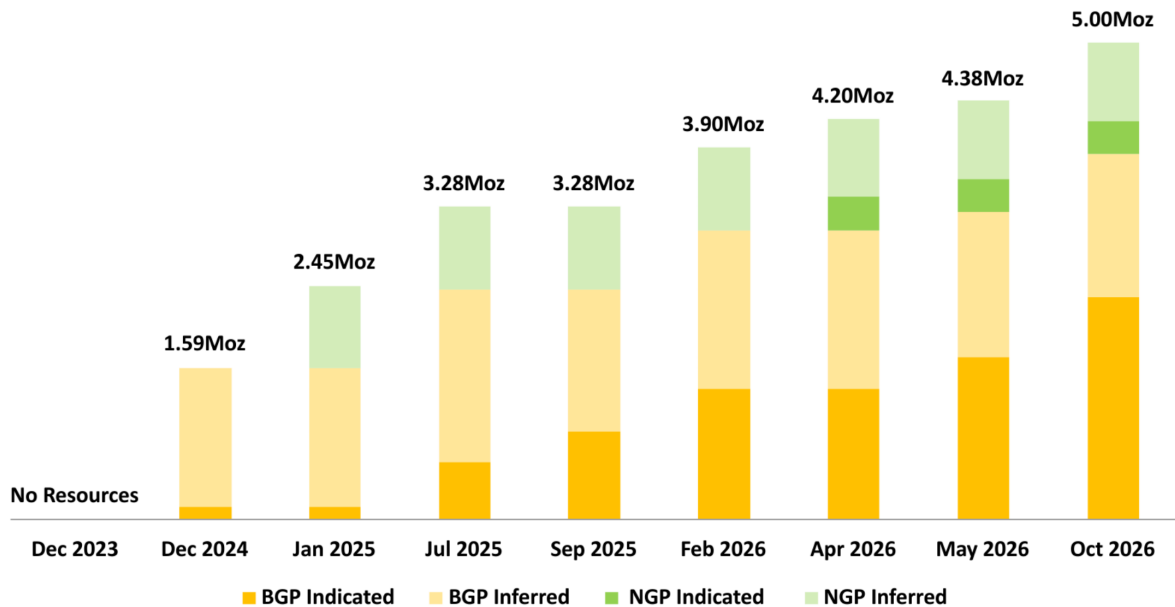
Figure 2: Aurum's Group Mineral Resource growth timeline 2
