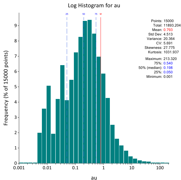
Figure 6: Log histogram for BST1 composites (all)
