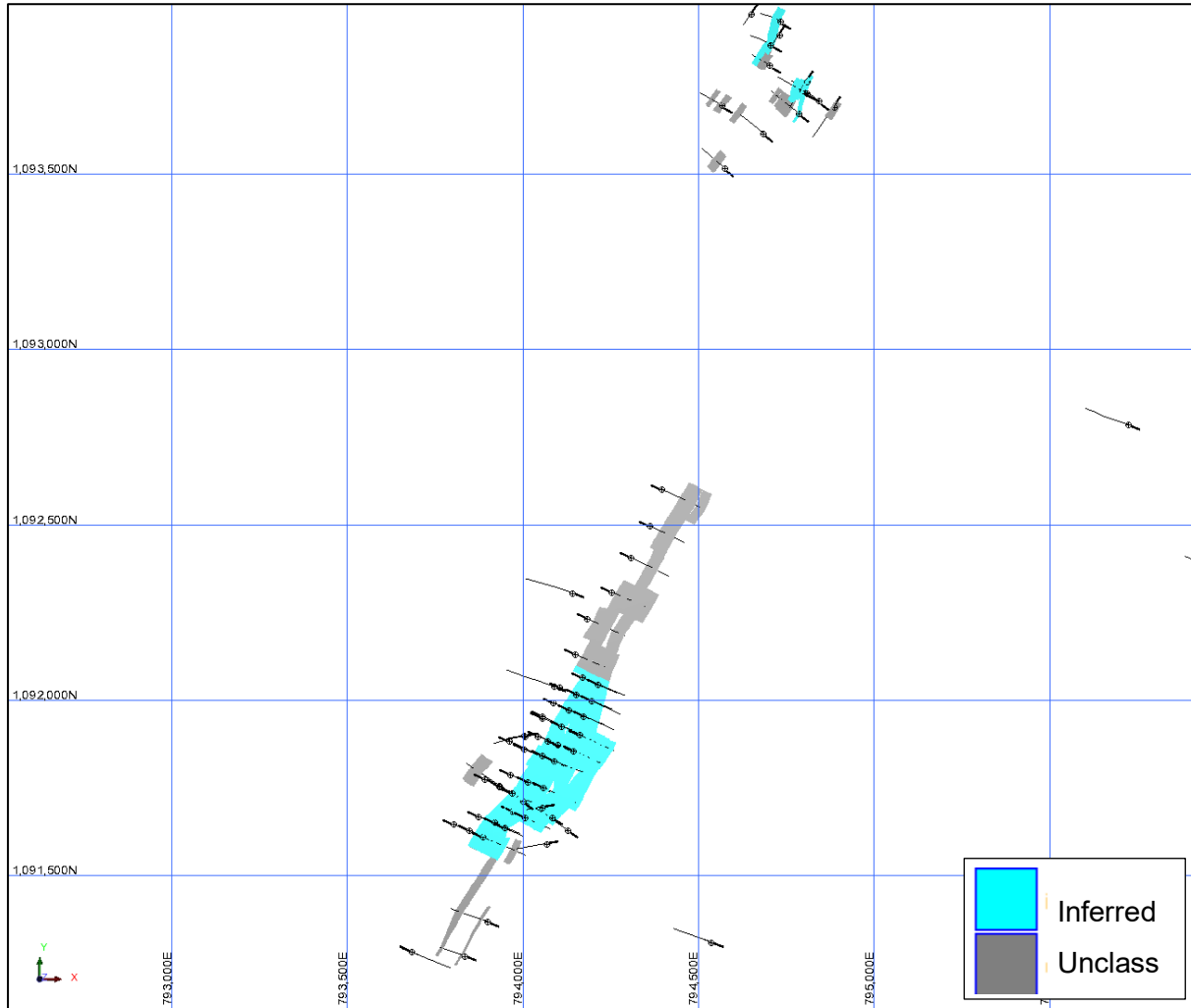
Figure 23: Plan view of BMT2 showing model classification (projected to surface with informing drilling)
