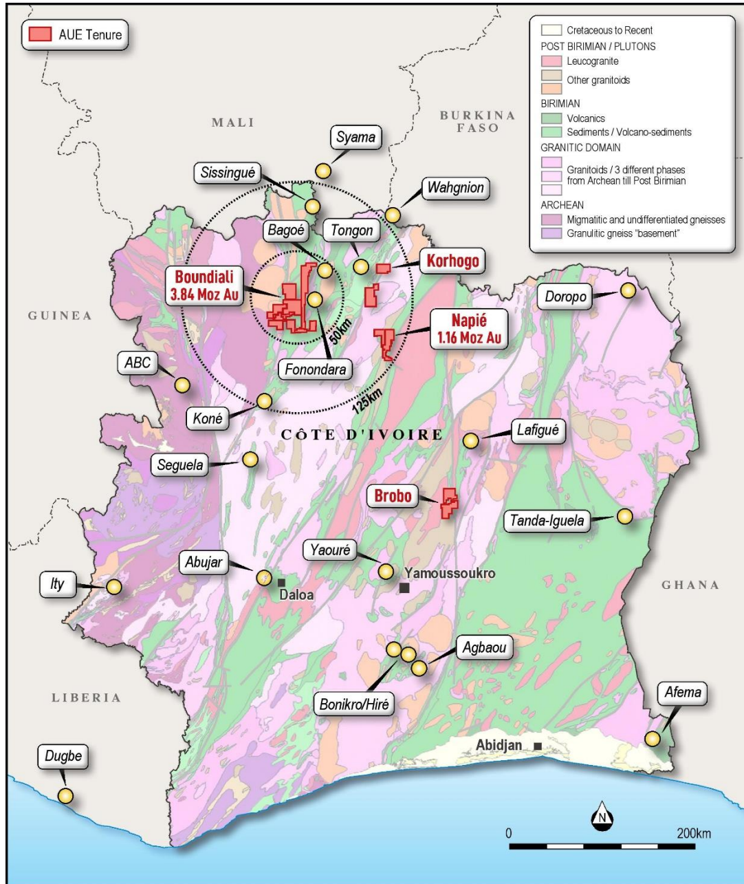
Figure 3: Location of Aurum's Boundiali Gold Project in Côte d'Ivoire
