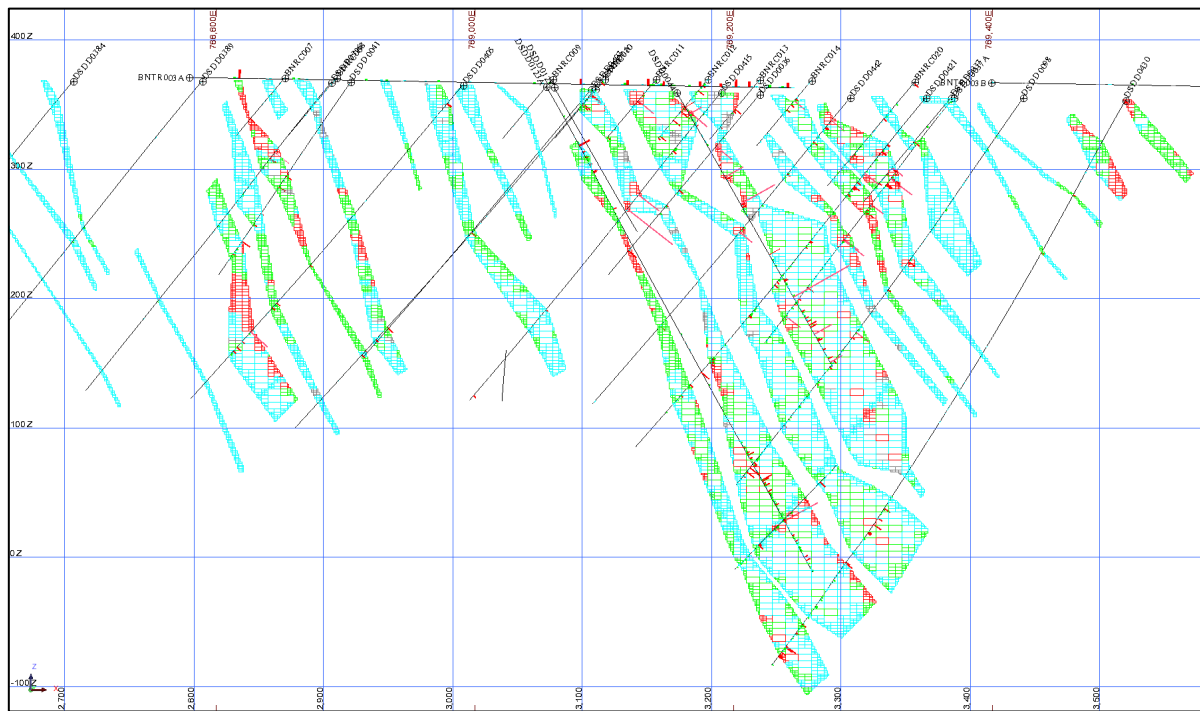
Figure 25: Example cross section (1,059,625mN) BDT2 showing estimated gold grades and drill data (looking north +/-25m)
