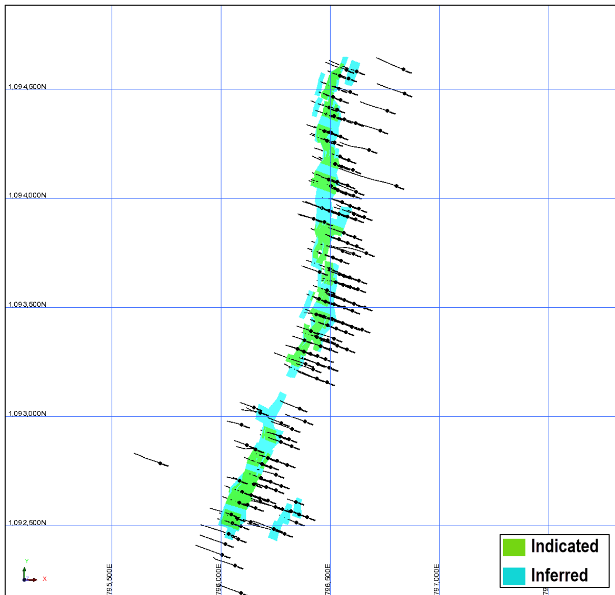
Figure 22: Plan view of BMT1 showing model classification (projected to surface with informing drilling)
