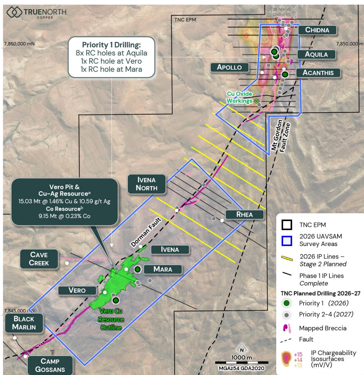
Figure 3. Geophysical survey lines targeting Rhea, Ivena North and extensions to the Aquila–Apollo mineralised system.
