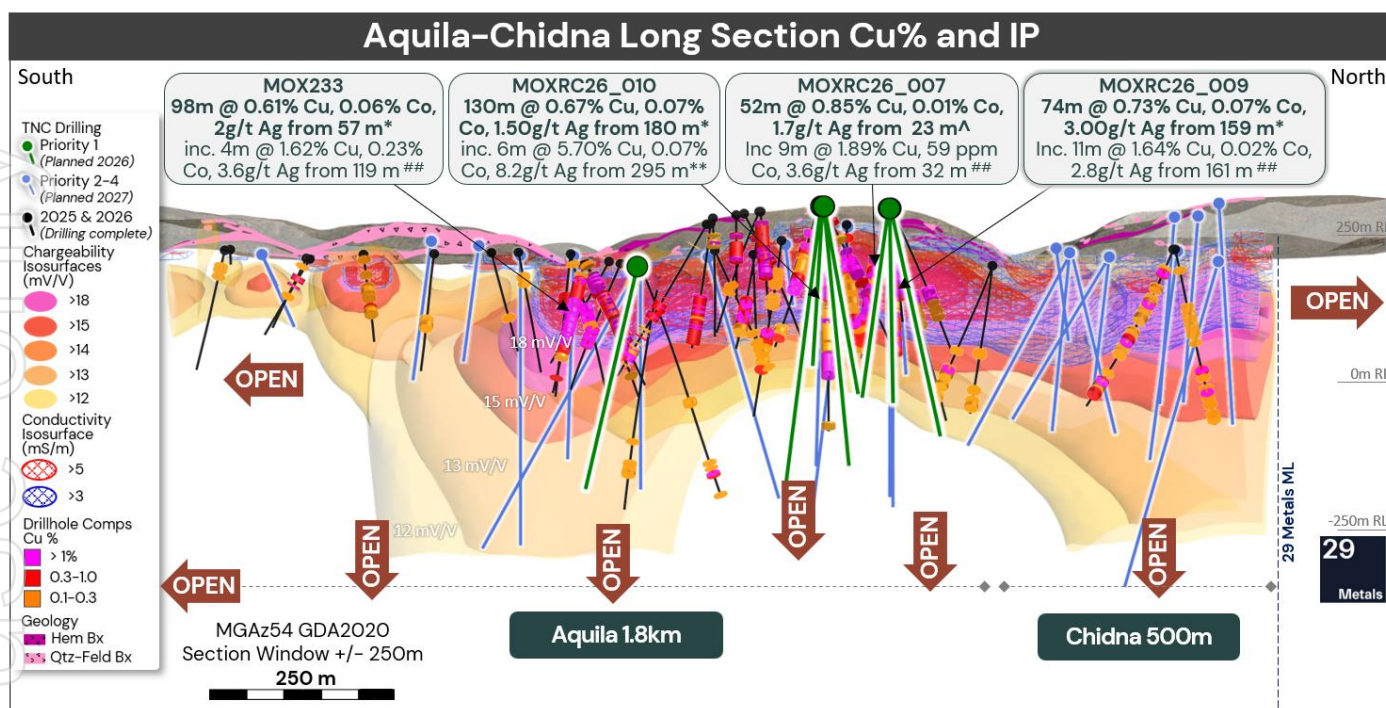
Figure 1. 2026 Phase 2 drilling targeting depth extensions at Aquila towards potential maiden Resource in 2027.
