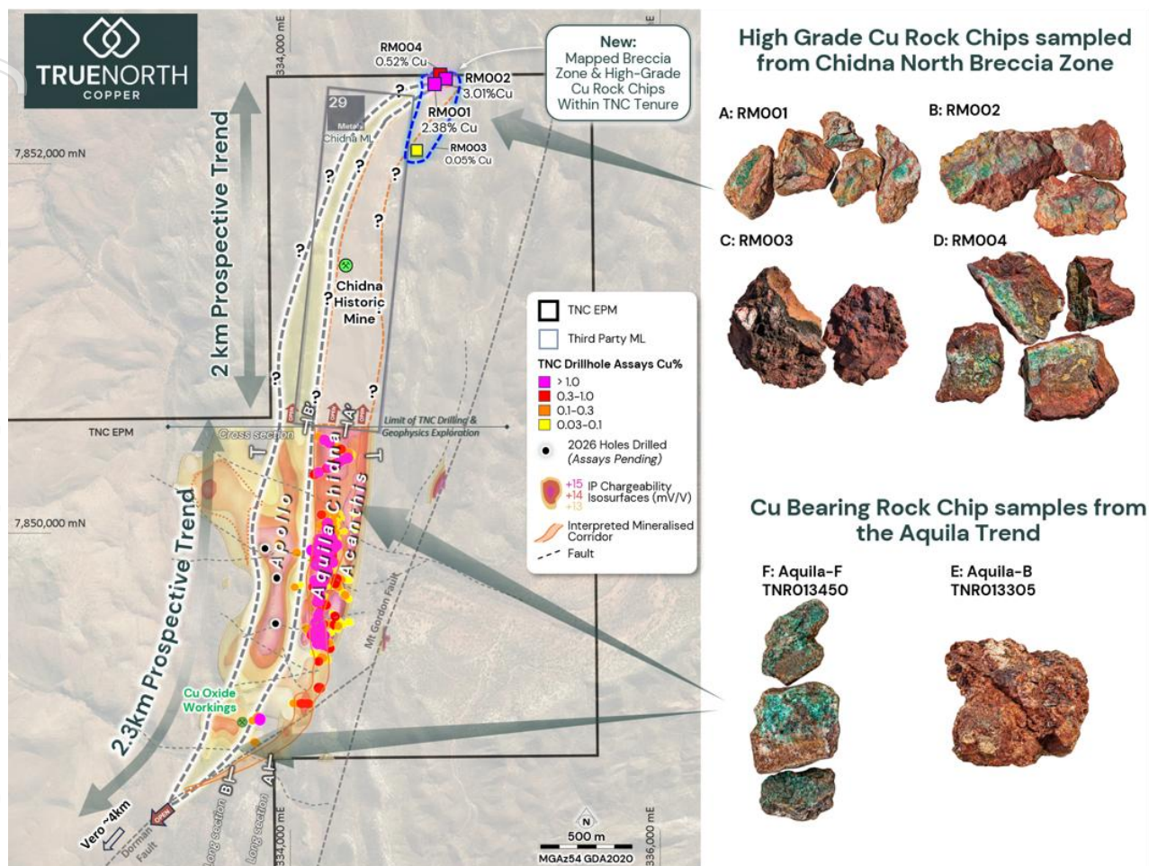
Figure 2. 2025 Aquila Discovery Rock Chips and 2026 Chidna North Rock Chips and 4km identified structure.
