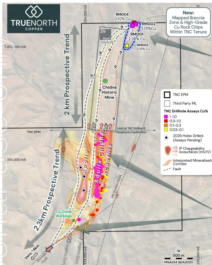
Figure 5. 2025 Aquila discovery rock chips 2026 Chidna North rock chips and 4km identified structure.
