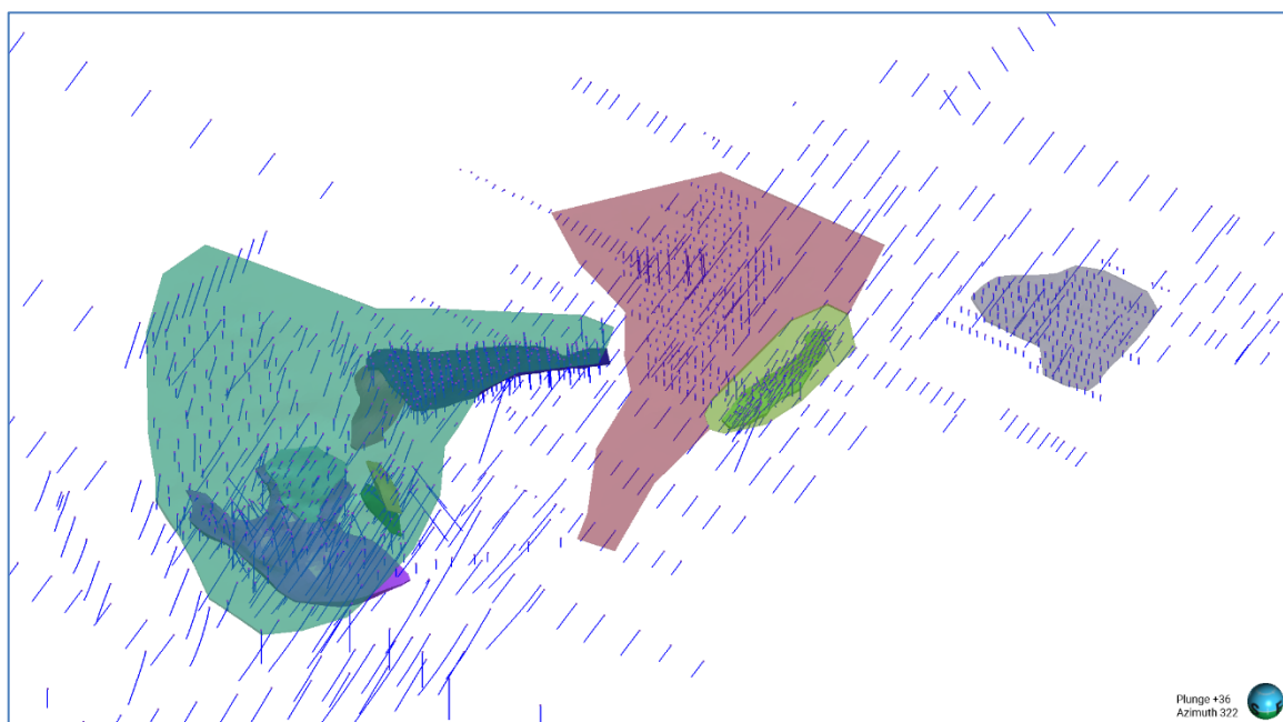
Figure 4: Perspective View of Model Wireframes and Drilling Data
