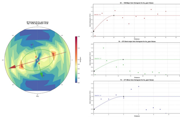
Figure 7: Variogram Models
