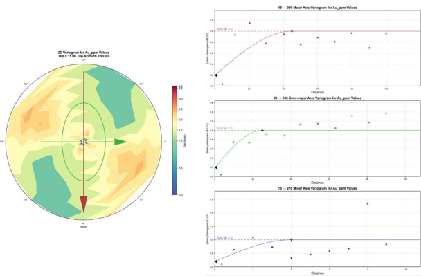
Figure 7: Variogram Models
