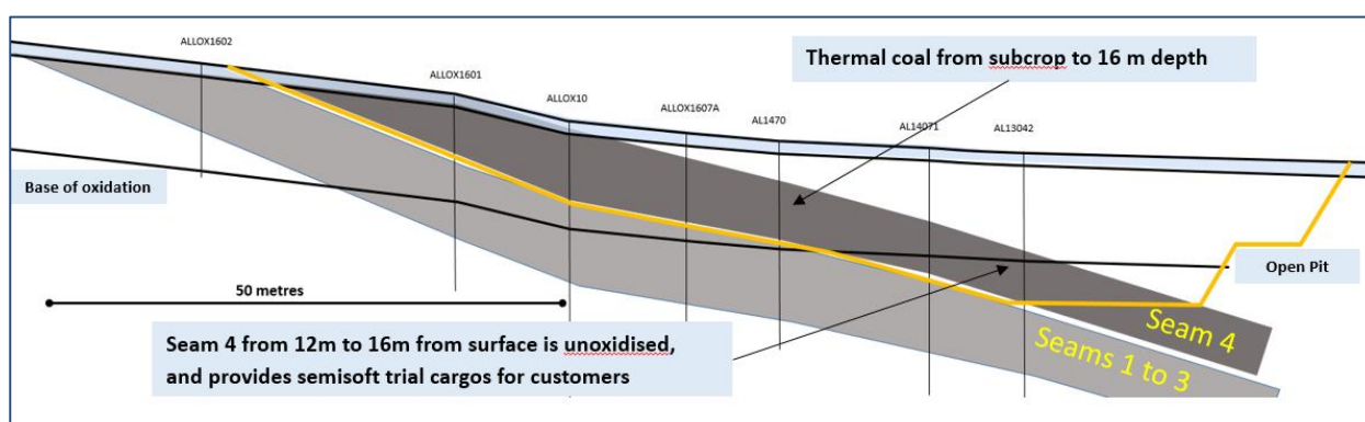
Figure 1 Typical cross section through Project F showing coals targeted for Phase One production
