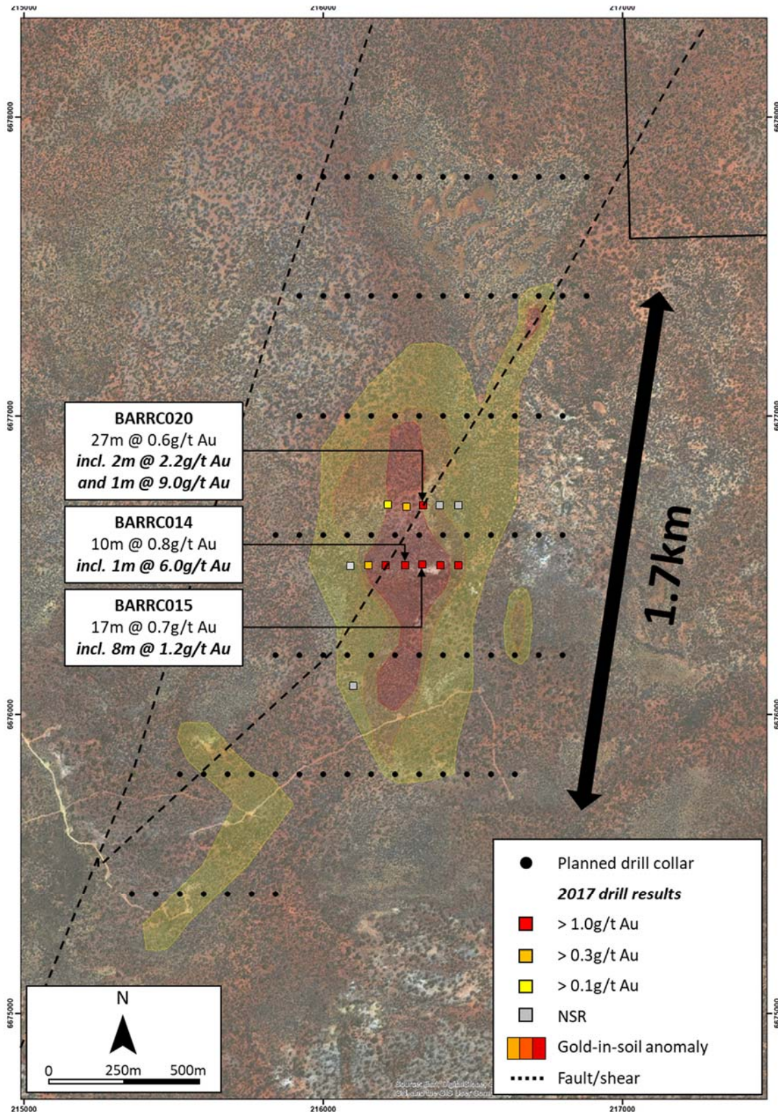
Figure 3 – T8 Prospect with 2017 drill results, gold-in-soil anomaly and planned aircore drill collar locations
